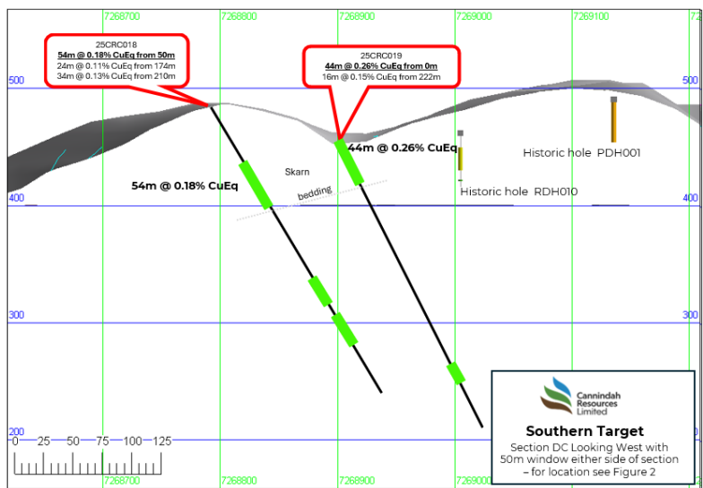
Figure 3: Cross section showing drill holes 25CRC018 and 25CRC019. Copper intervals are associated with skarn development.
