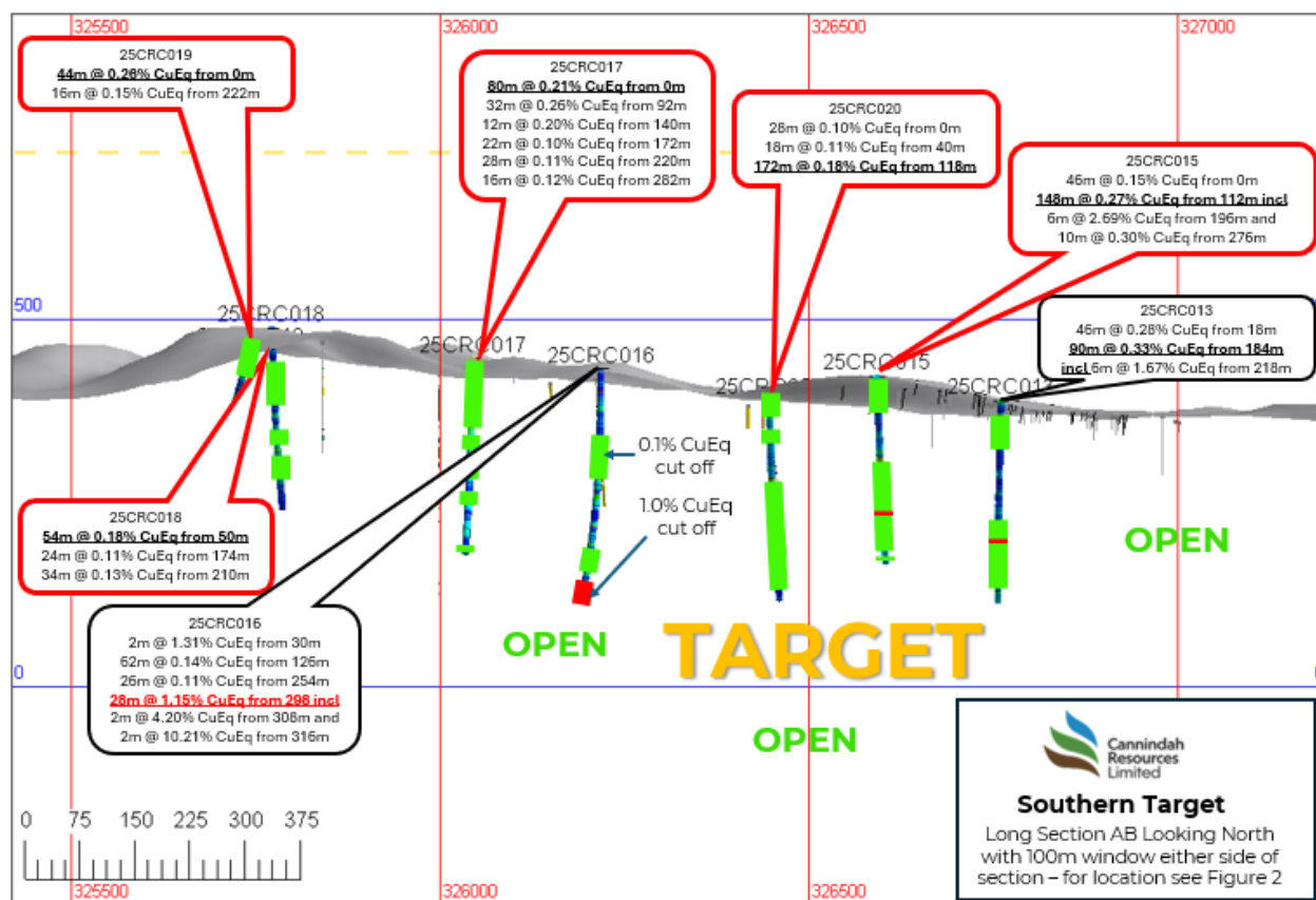
Figure 6: Long section looking north of 2025 drilling with all drill results.
