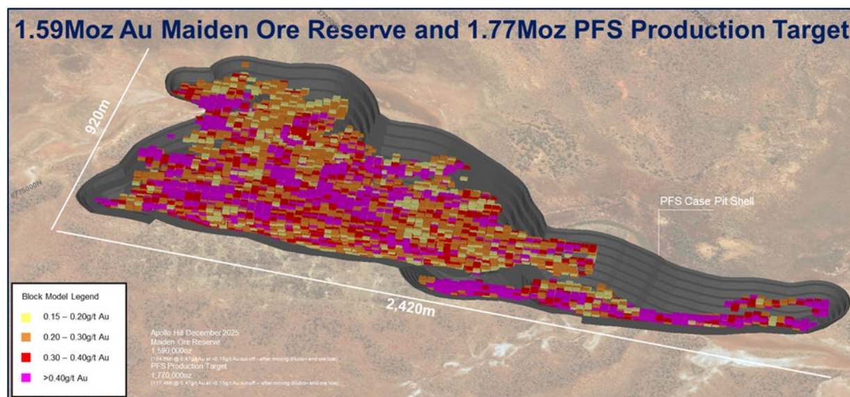
Figure 1: Apollo Hill Gold Project: PFS Final Mine Design – Production Target of 117.4Mt at 0.47g/t for 1.77Moz 4 .
