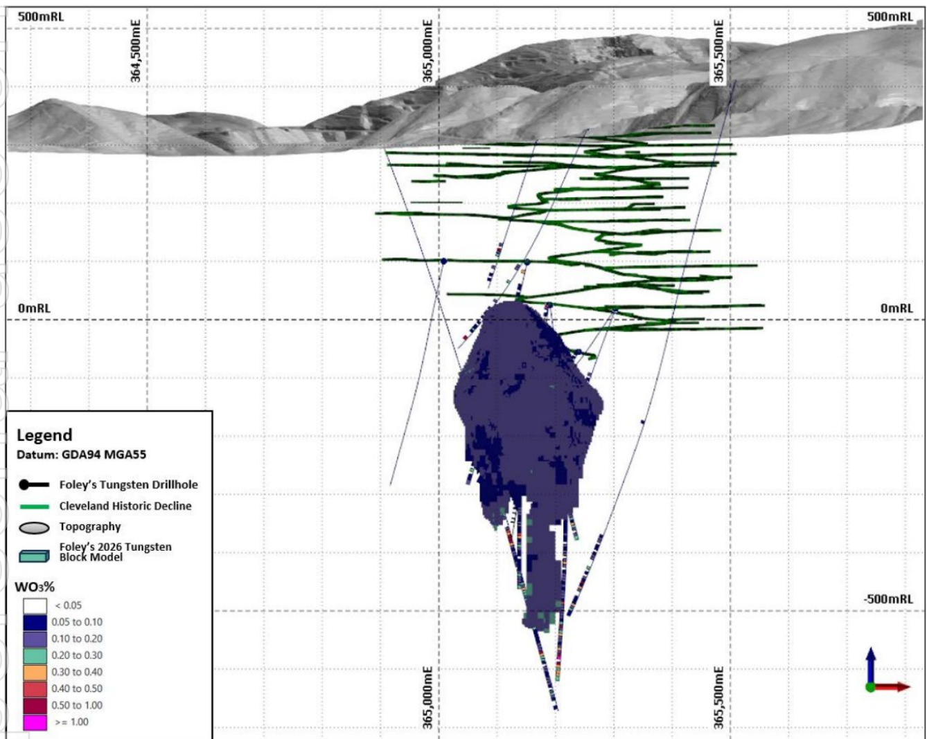
Figure 4. Foley Zone tungsten Mineral Resource Block Model with topography and historical Cleveland Mine underground workings.
