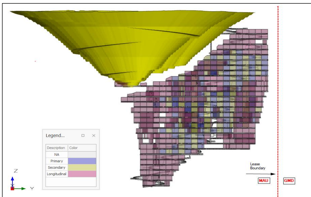
Figure 3: LJN4 Underground Design, view looking west
