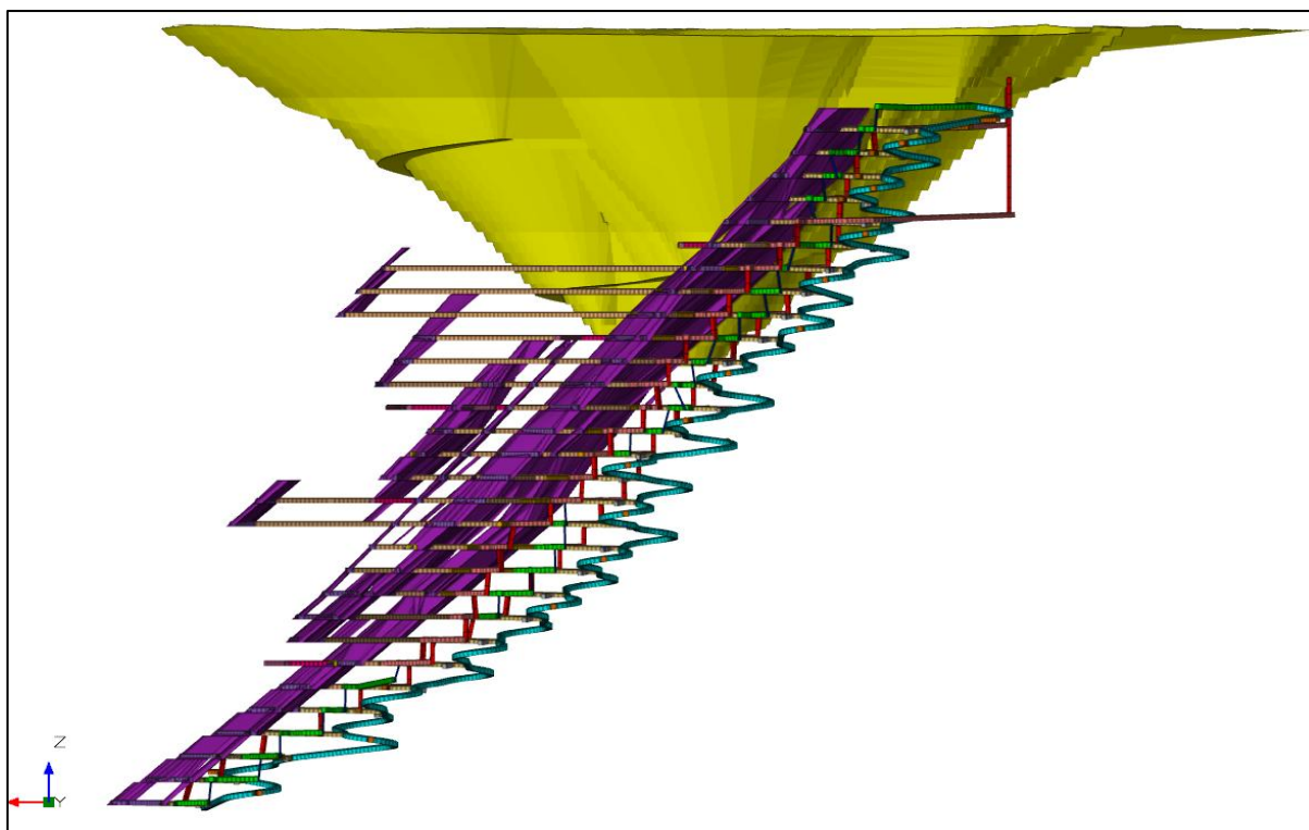
Figure 4: LYN4 Underground Design, view looking south
