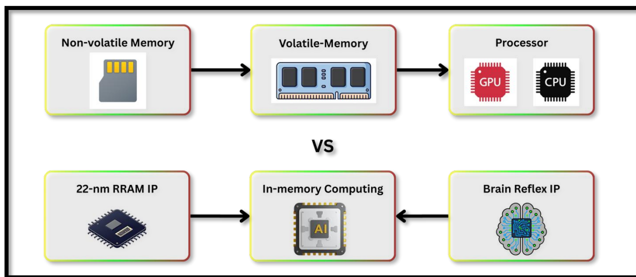
Figure 2: A conceptual comparison of data-movement-heavy traditional computing architectures versus a 22-nm RRAM-enabled neuromorphic in-memory computing approach.
