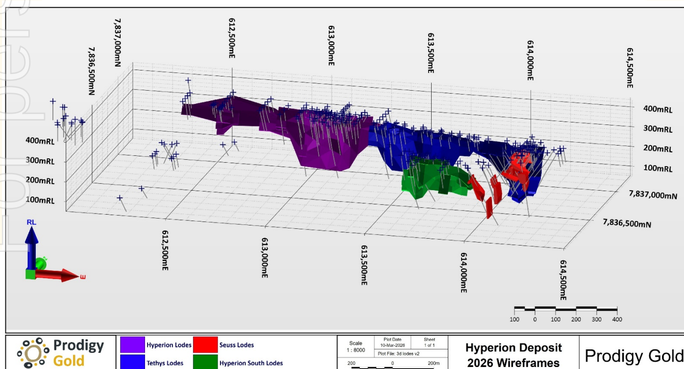
Figure 3 Hyperion mineralisation showing location of lodes used in modelling
