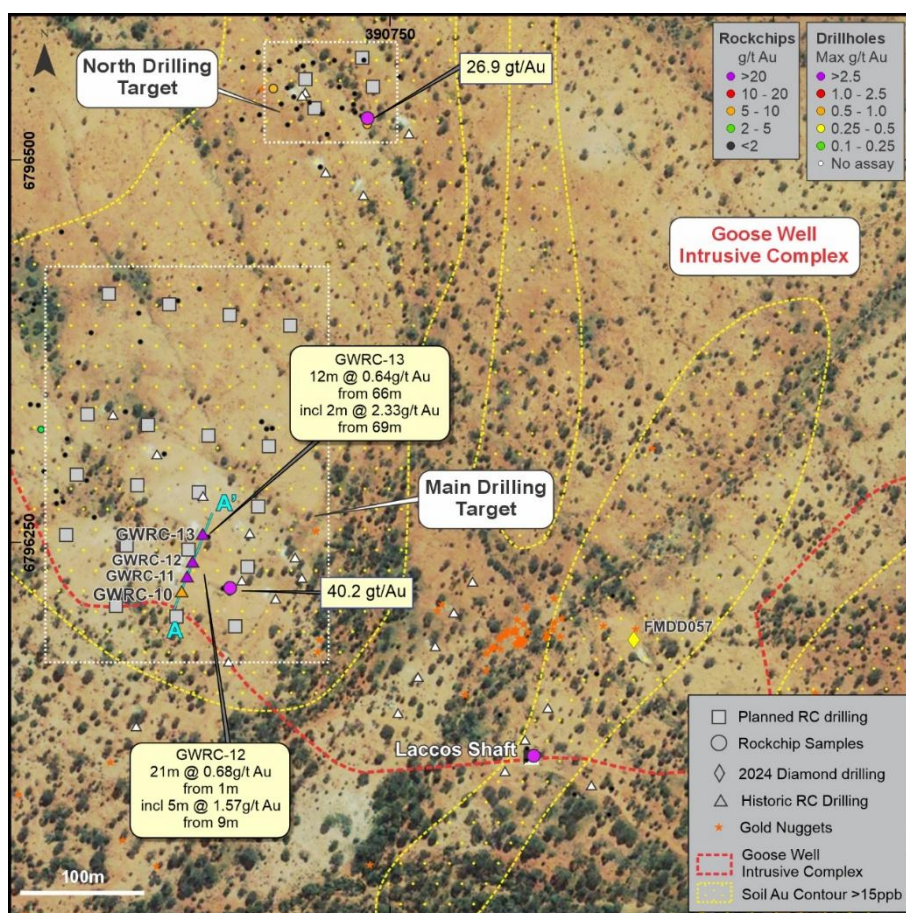
Figure 3 Aerial imagery at Goose Well prospect with Maiden RC Program's planned drill holes. Figure also highlights the gold-in-soils contours with coincident high grade rock chips and historic drilling.
