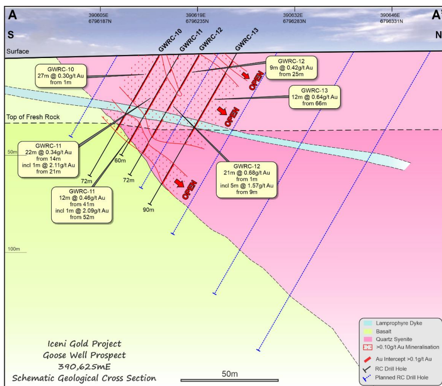
Figure 4 Goose Well drill section showing results from resampling of 2014 era RC drillholes, with interpreted geology, key intercepts and planned holes from the Maiden RC Drill Program
