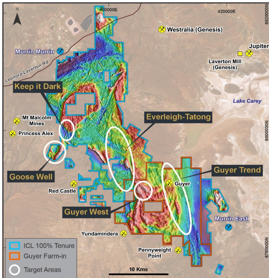
Figure 1 TMI Aeromagnetic Image (warm colours represent stronger magnetic signature) of the 14MWGP Area with key target areas (Goose Well target in the project's far west). Refer to Figure 2 for RC Drill Program details.
