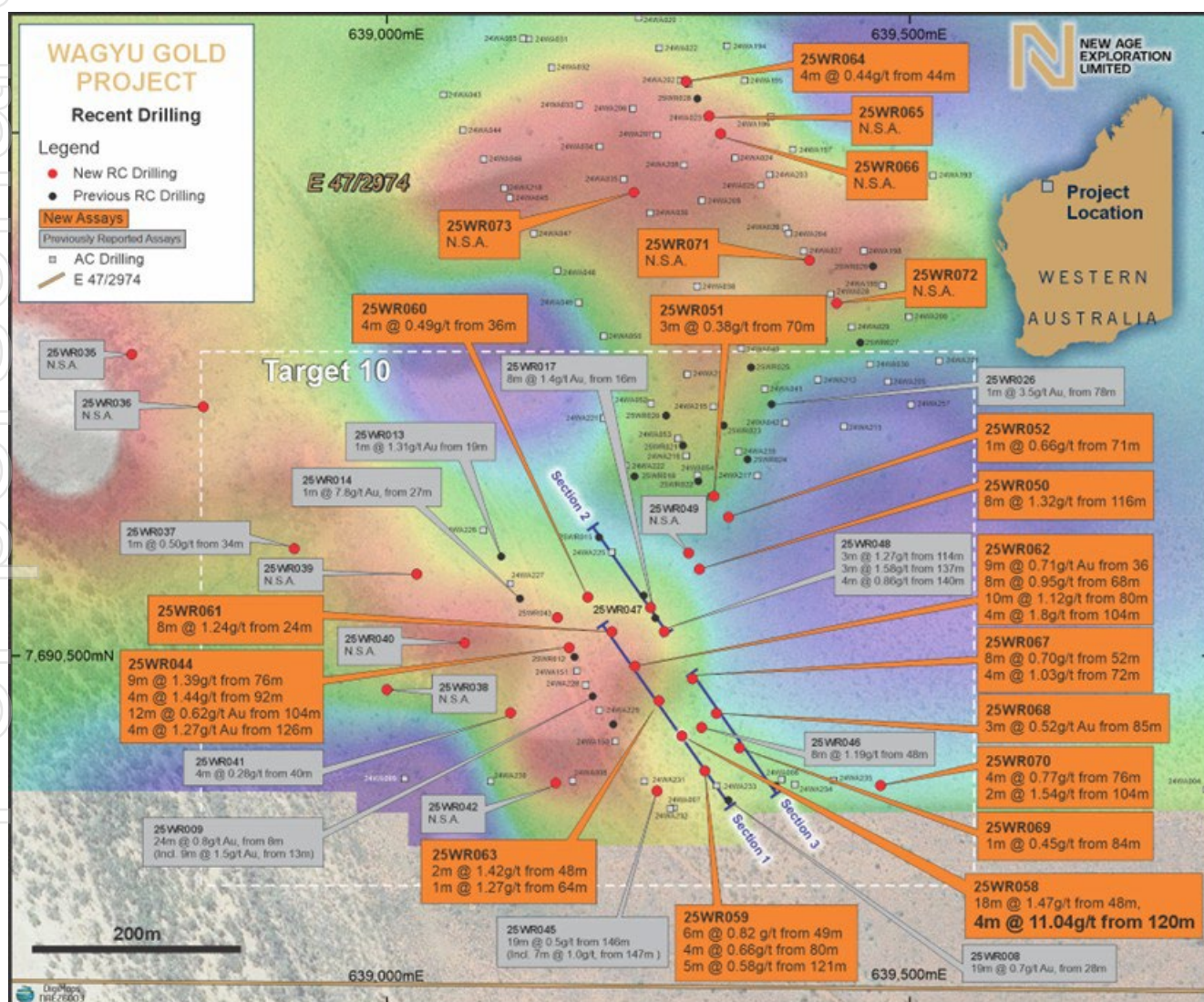
Figure 1: Wagyu Gold Project, Target 10. Collar plot with significant new RC drill intersections. Maximum downhole gold assay result shown for new assays (orange boxes) and previously reported results (grey boxes). Background colour is ground gravity data.
