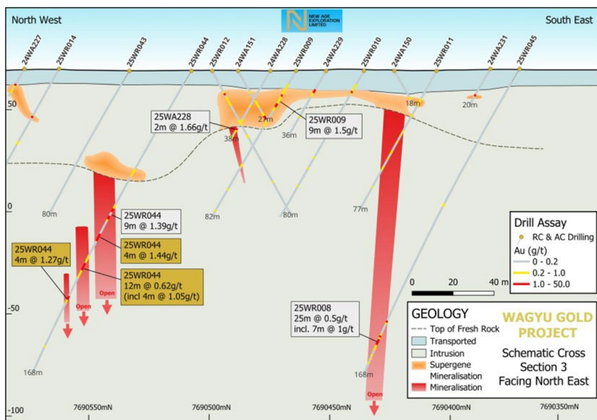
Figure 4: Cross section 3 - Target 10
