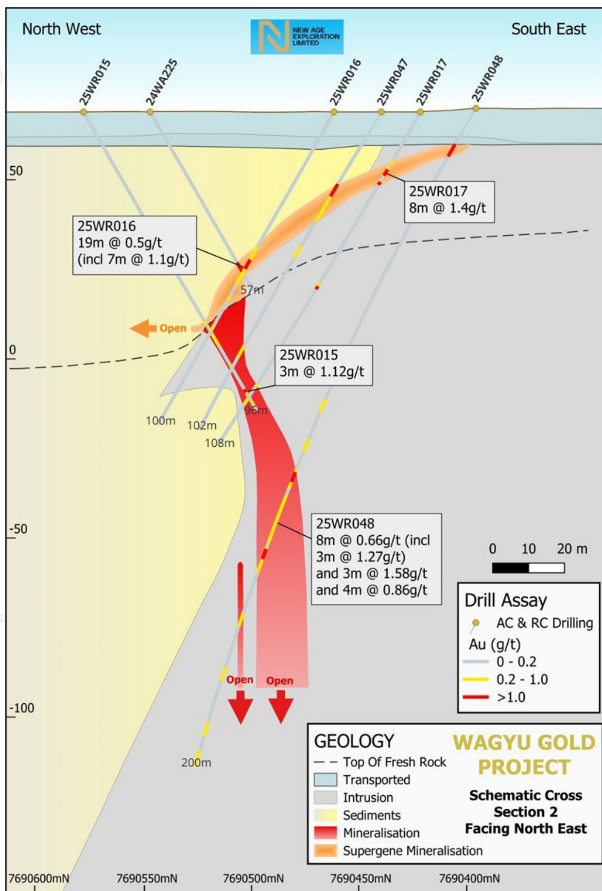
Figure 3: Cross section 2– Target [10]
