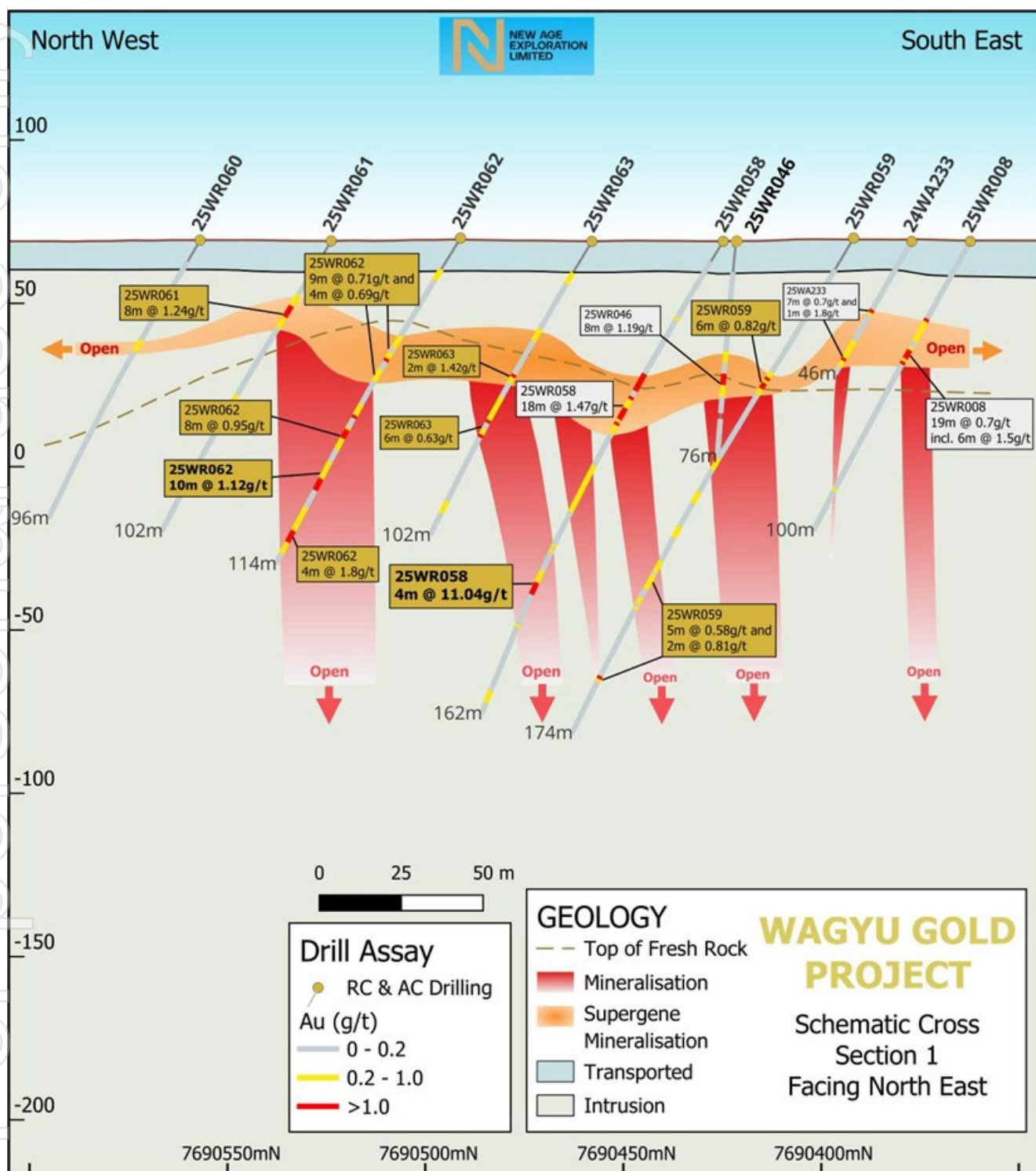
Figure 2: Cross section 1– Target 10.
