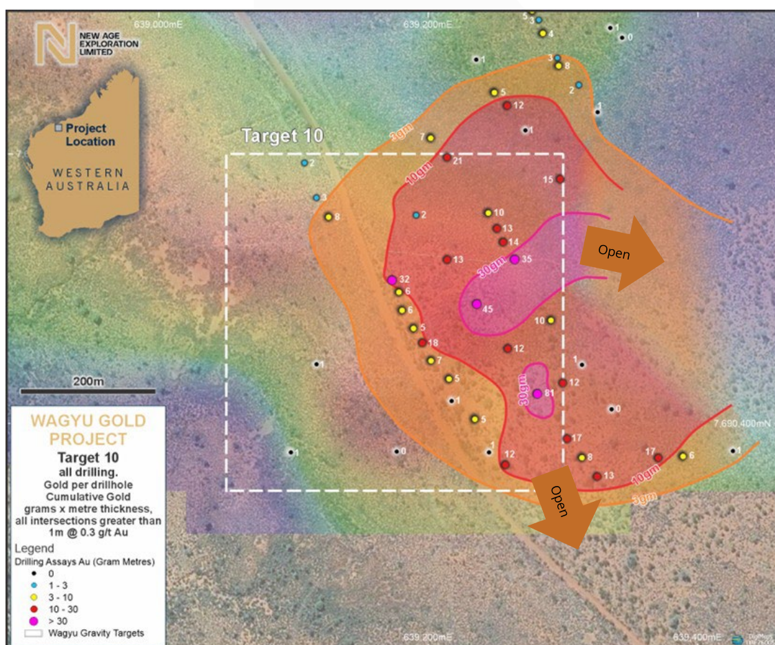
Figure 5: Wagyu Gold Project. Target 10, contour plan of gold per drillhole, Grams x Metres.
