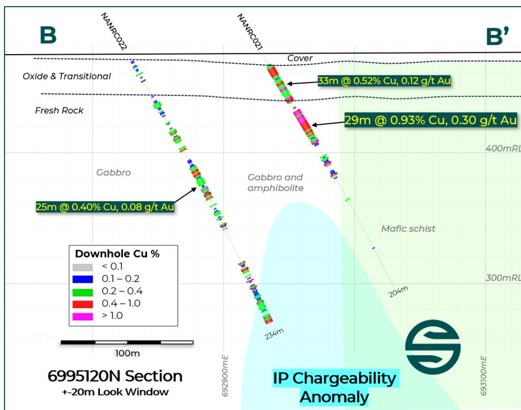
Figure 4. Nanadie Project cross-section 6995120N showing Phase 1 step-out drillholes NANRC021 and NANRC022, simplified geology, and outline of a 2025 IP chargeability anomaly.
