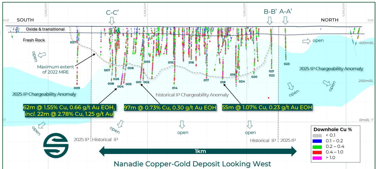
Figure 2. Nanadie long section looking west, showing all Phase 1 drillholes labelled, high grade intercepts 3 , southern IP chargeability anomaly 2 , and location of cross-sections A-A', B-B' and C-C' in this release relative to the maximum extent of the 2022 MRE block model and historical drilling 1 .
