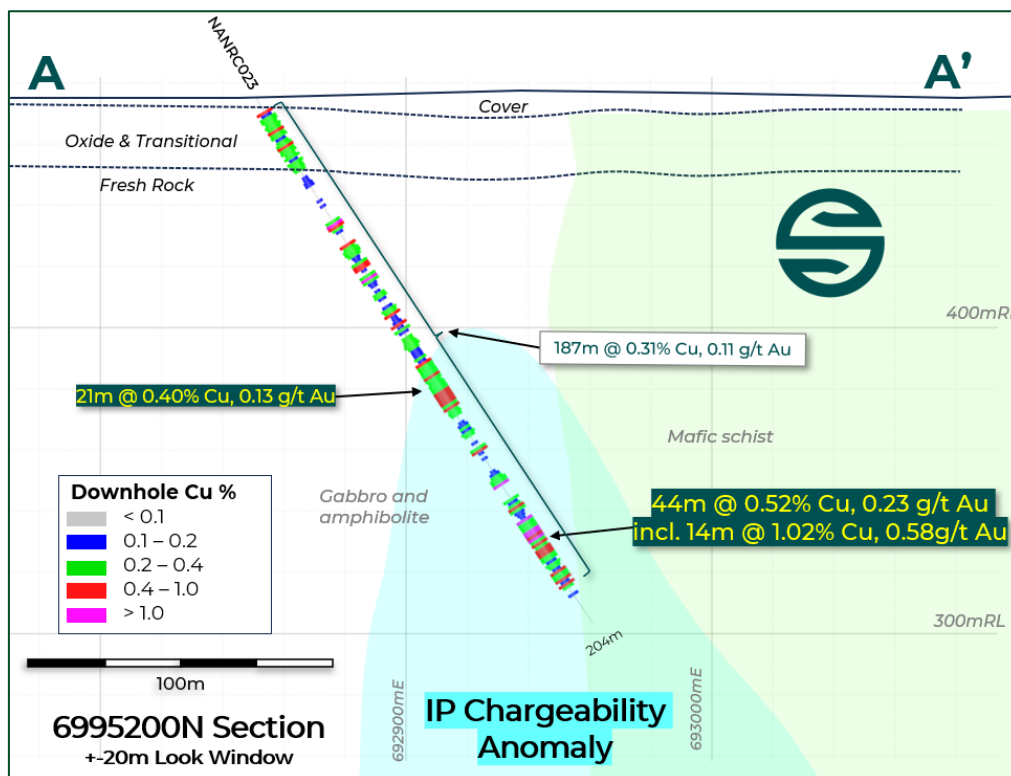
Figure 3. Nanadie Project cross-section 6995200N showing Phase 1 step-out drillhole NANRC023 simplified geology, and outline of a 2025 IP chargeability anomaly.
