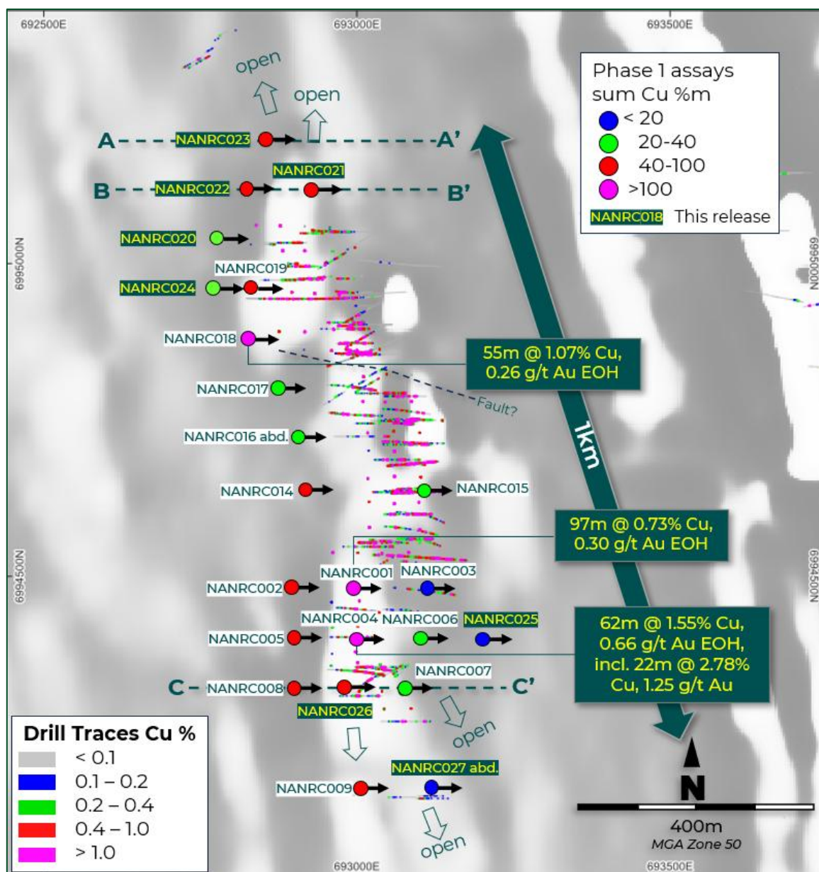
Figure 1. Nanadie Deposit aeromagnetic imagery showing Phase 1 RC drill collars (coloured for sum of Cu% metres downhole) and high-grade intercepts 3 , and downhole copper values in all previous drilling 1 , projected to surface. Cross-section A-A' labelled. Collars this release in yellow font.
