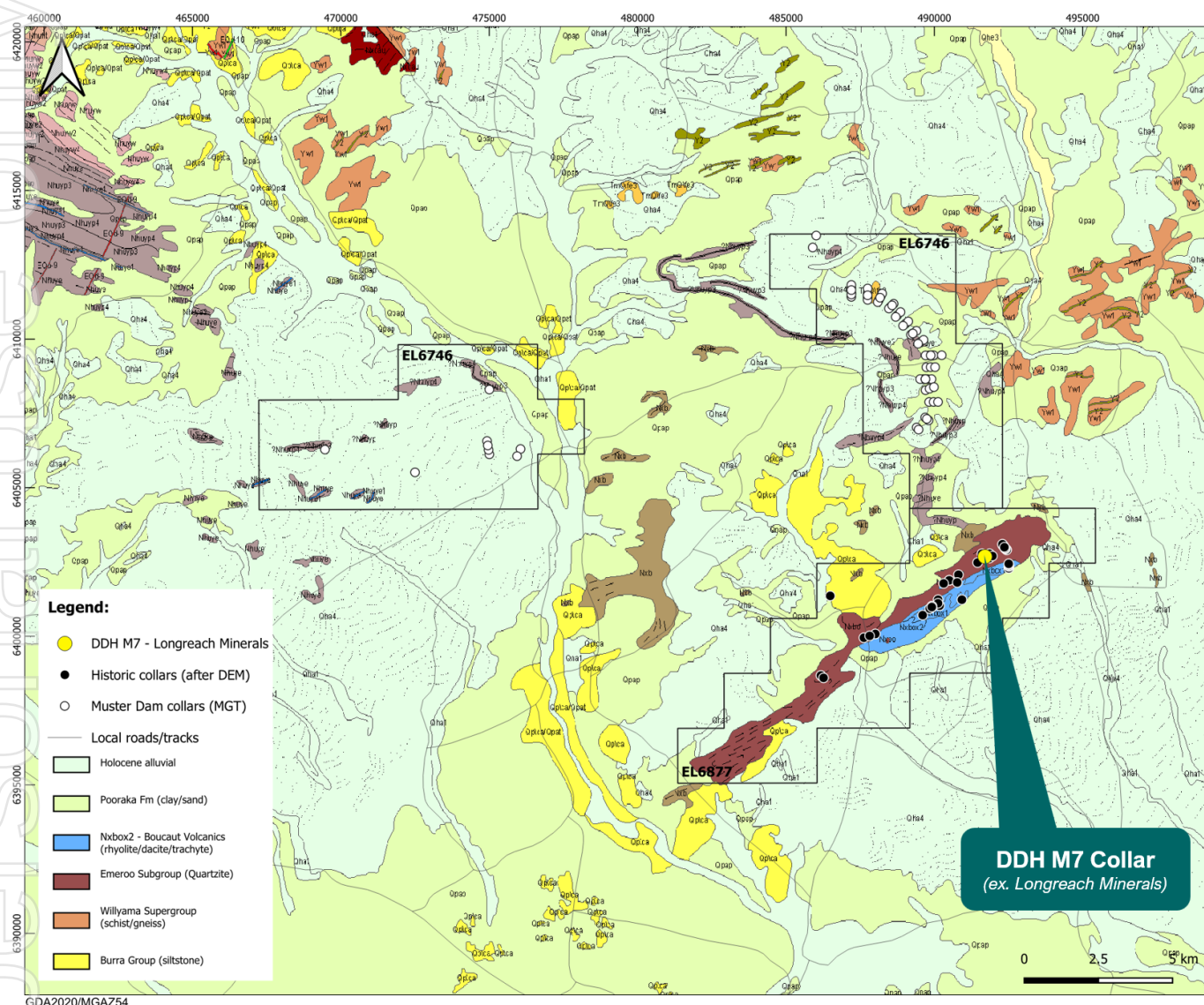
Figure 5. Local geological units – 100K mapping (after DEM-SARIG)
