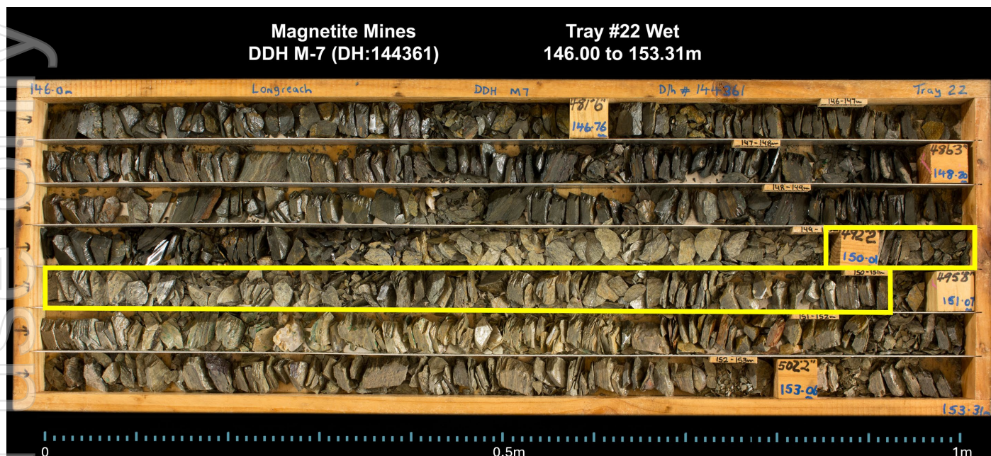
Figure 1. DDH M7 diamond drill core, NQ diameter 47.6mm, 146 to 153.31 metres, zone of mineralisation. Intersection 150-151m highlighted yellow corresponds with assayed results of 63.2g/t silver and 2.8% copper.
