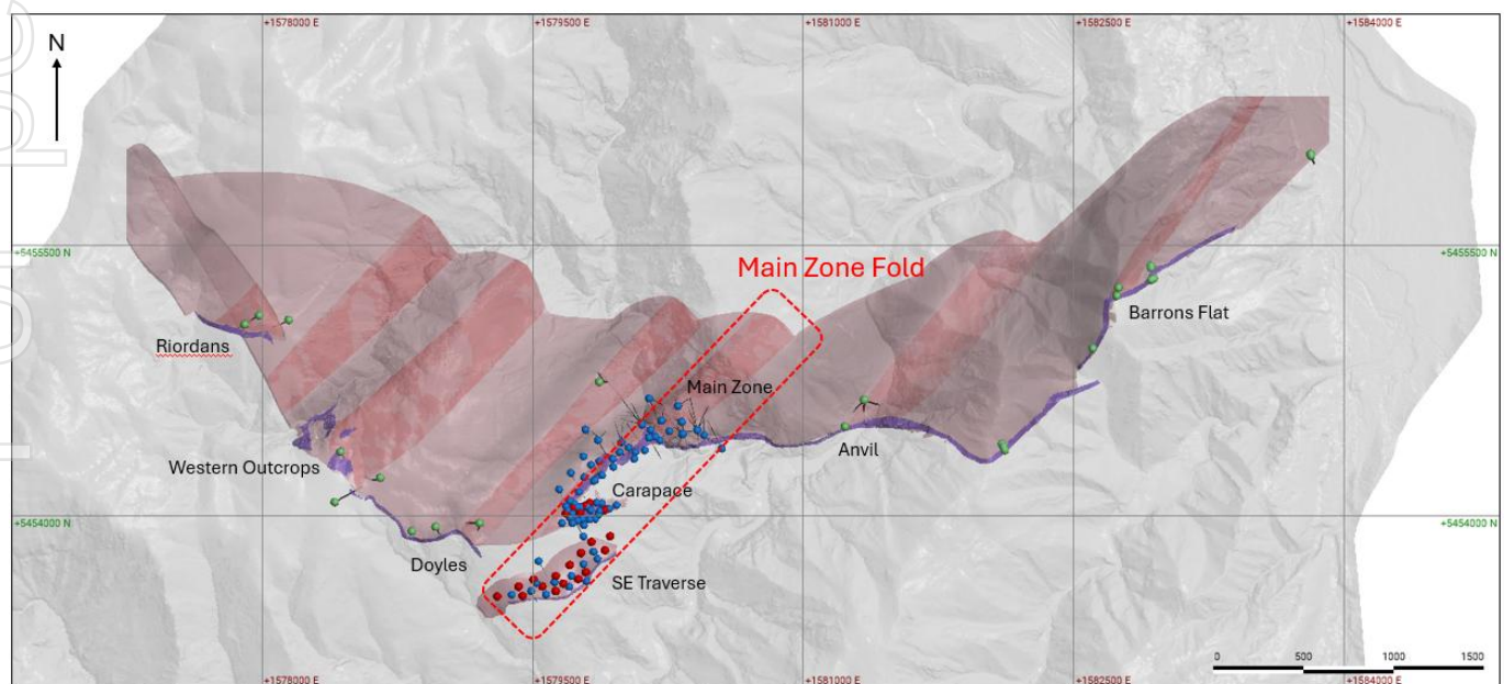
Figure 2: Isometric plan view showing north dipping SCD (light pink), interpreted NE plunging mineralised shoots (dark pink), drillholes used in the MRE (blue points), exploration holes (green points) and current infill drilling (red dots).
