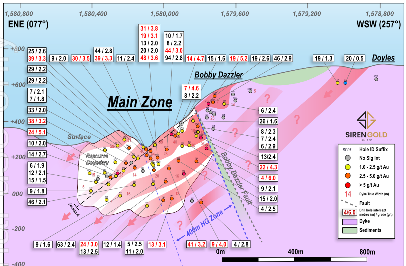
Figure 3: Isometric long section view showing north dipping SCD (light pink), interpreted NE plunging mineralised shoots (dark pink), drillhole intercept midpoints and MRE boundary (white)
