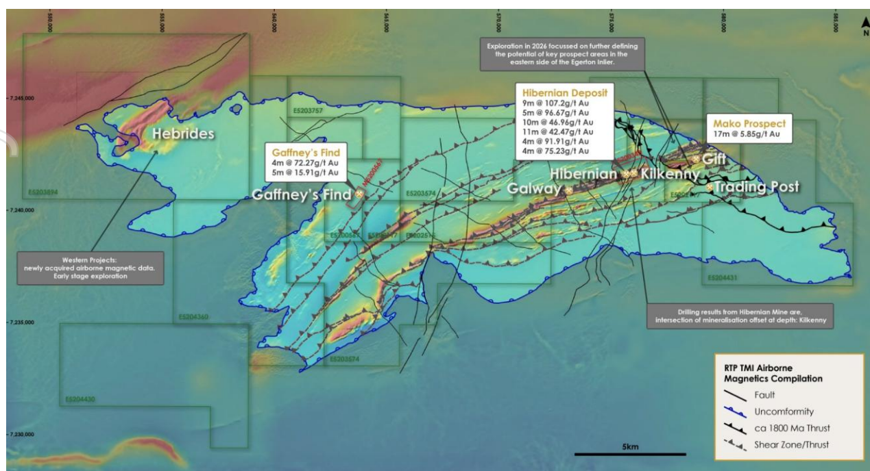
Figure 5. Regional geological overview of the Mt Egerton Goldfield.
