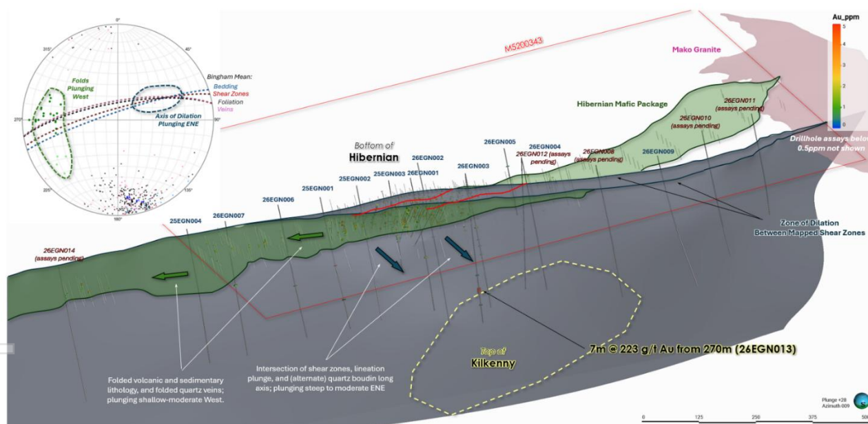
Figure 4. 3D oblique view of the of Mt Egerton Goldfields geology and structural interpretation with collar map.
