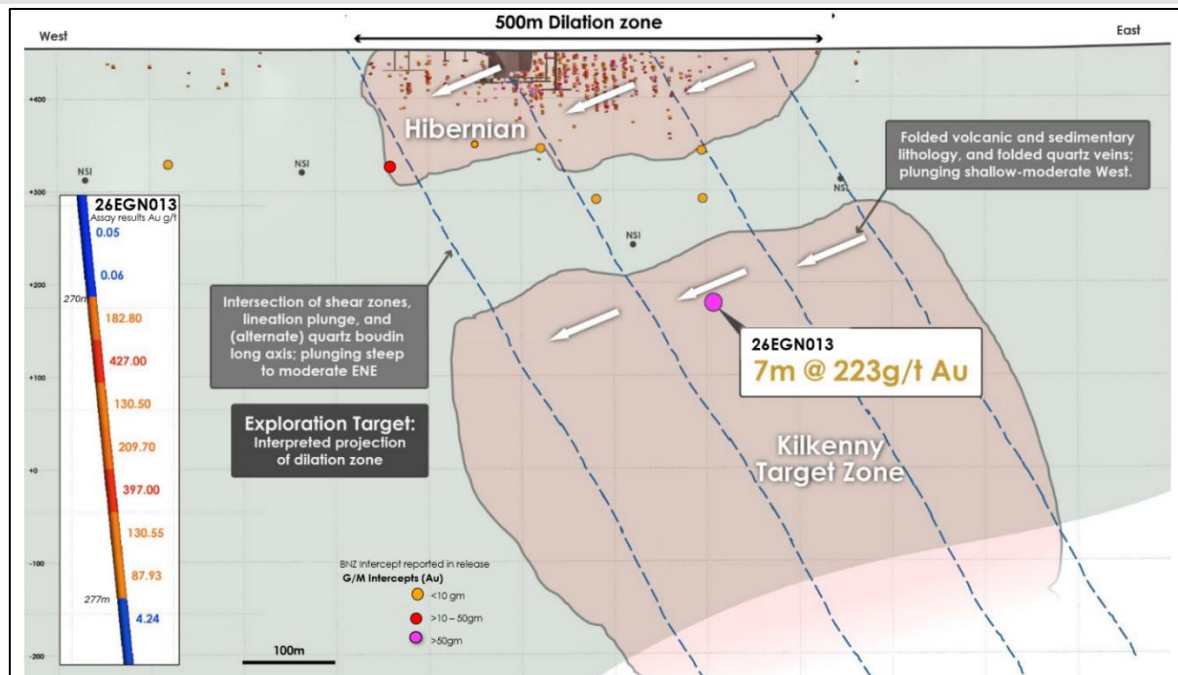
Figure 1. Long section of Kilkenny Discovery zone, showing structural controls. (note Kilkenny discovery offset out of the page below Hibernian).
