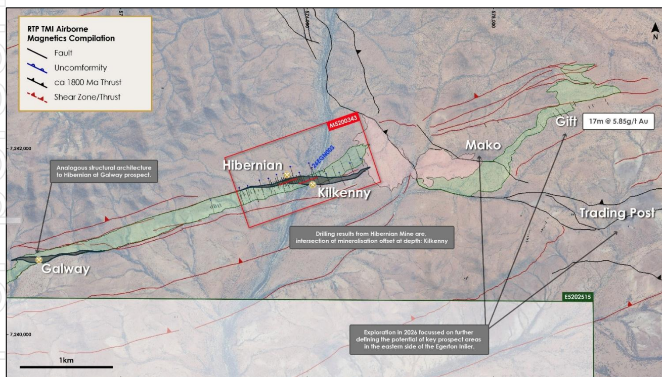
Figure 2. Plan view of Mt Egerton Goldfields geology and structural interpretation with collar map.
