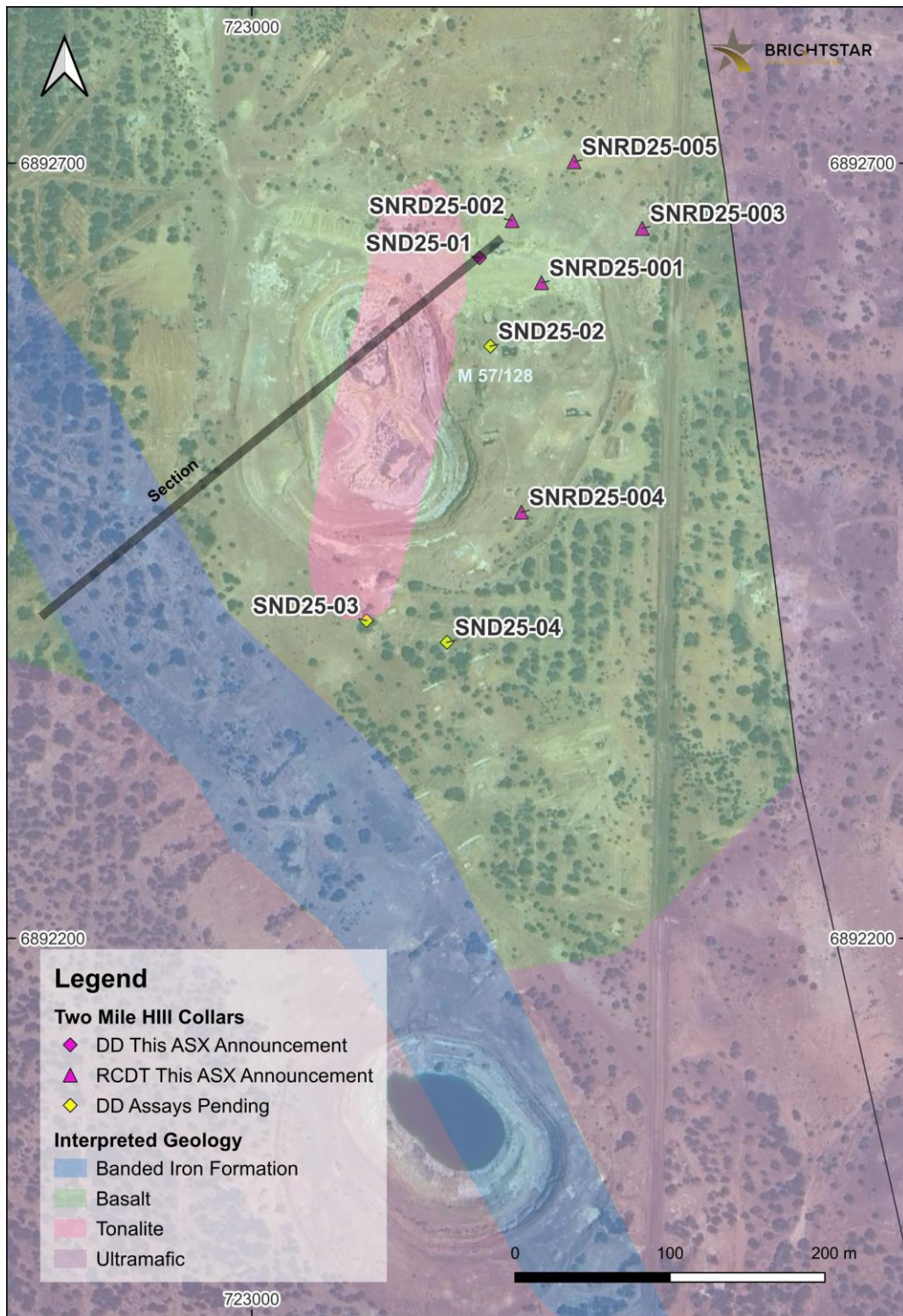
Figure 4: Plan view map of RC and Diamond drill collars for the Two Mile Hill-Shillington drilling
