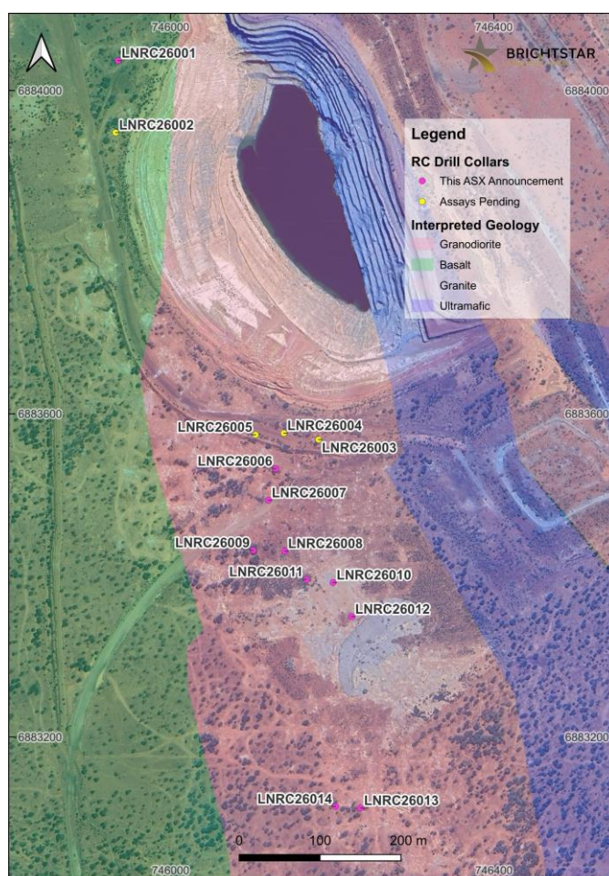
Figure 8: Plan view of RC and diamond drill collars completed at the Lord Nelson deposit
