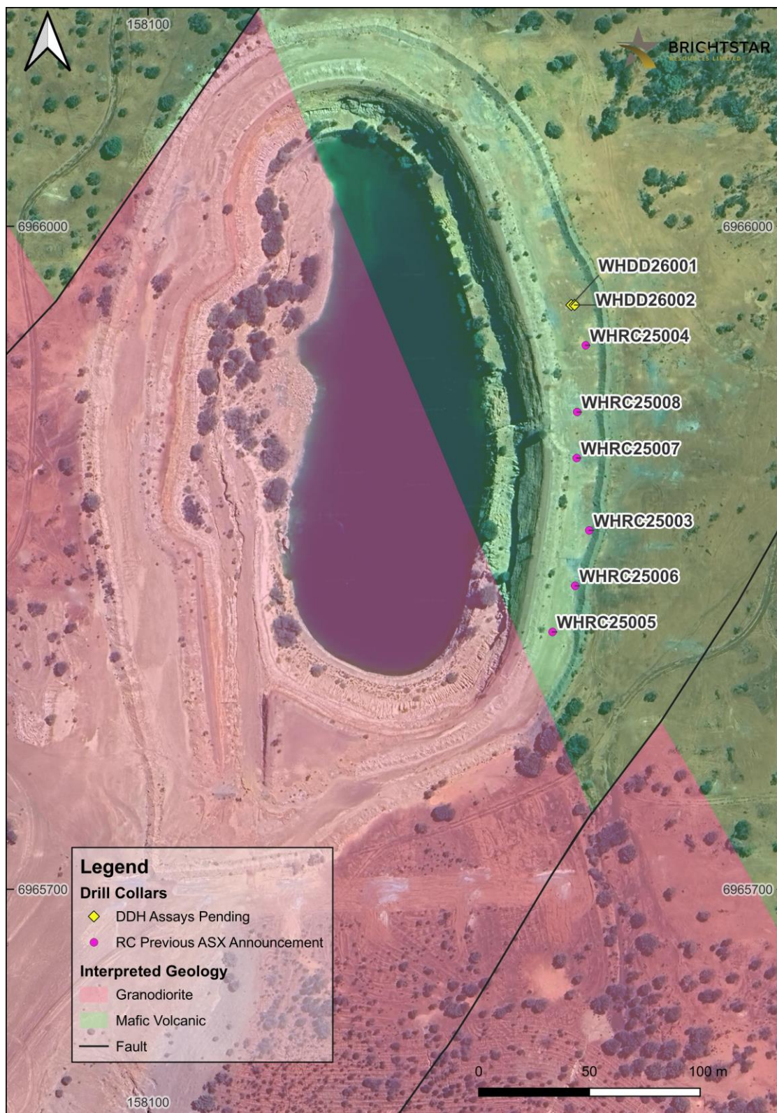
Figure 7: Plan view map of RC and DD drill collars for the Whistler drilling program
