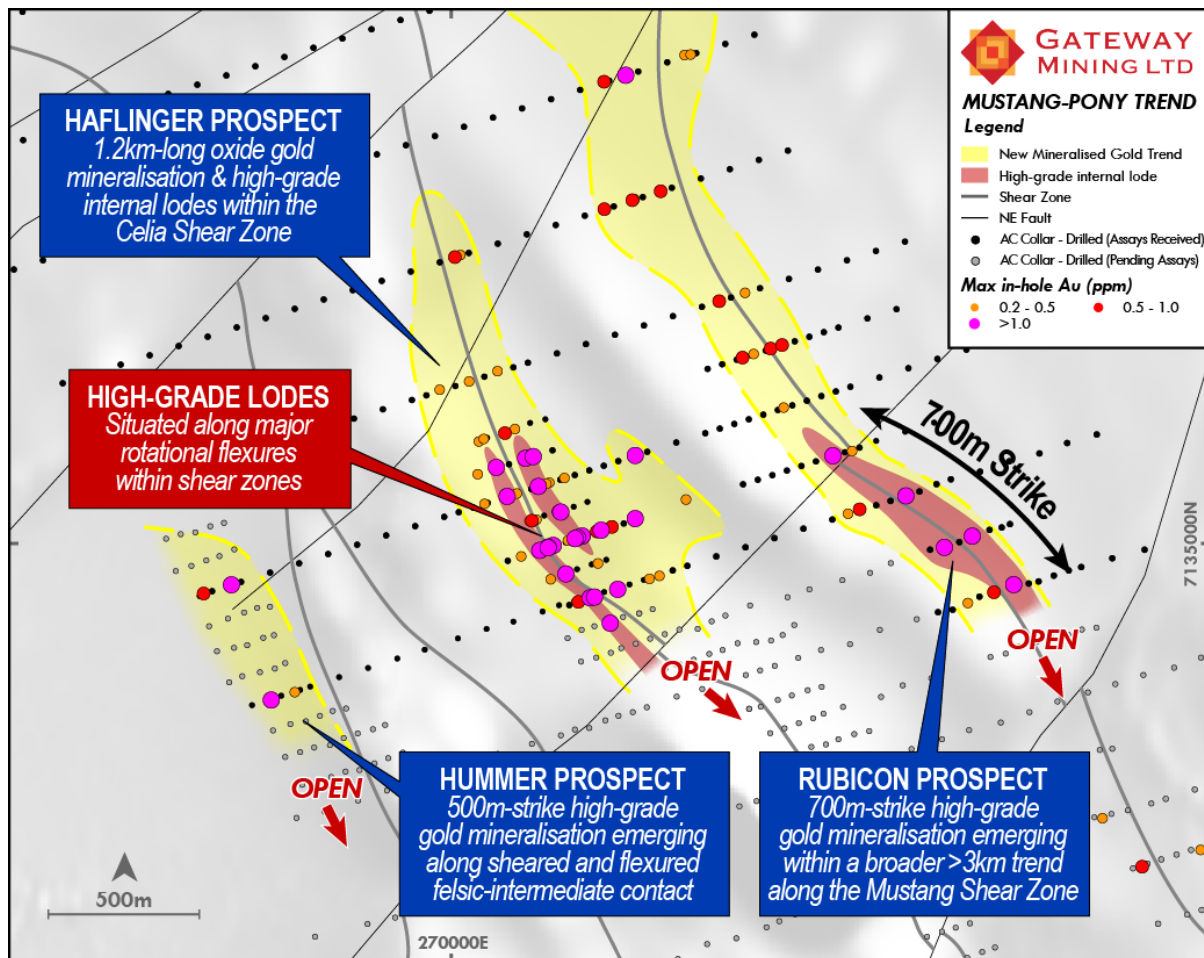
Figure 2: Zoomed in map showing the three parallel prospects, Hummer (west), Haflinger (centre) and Rubicon (east).
