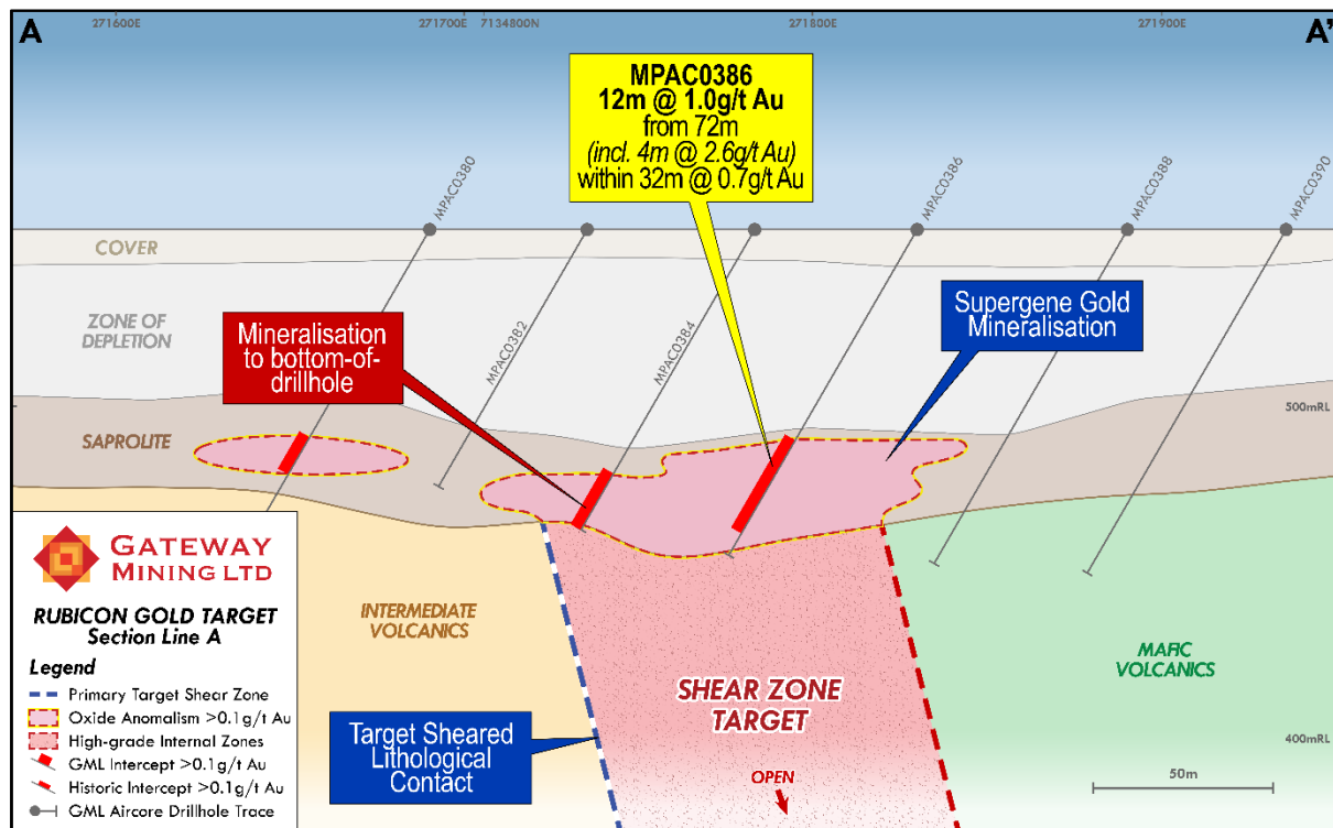
Figure 3: Rubicon Cross Section demonstrating the shear zone in fresh rock remains untested.
