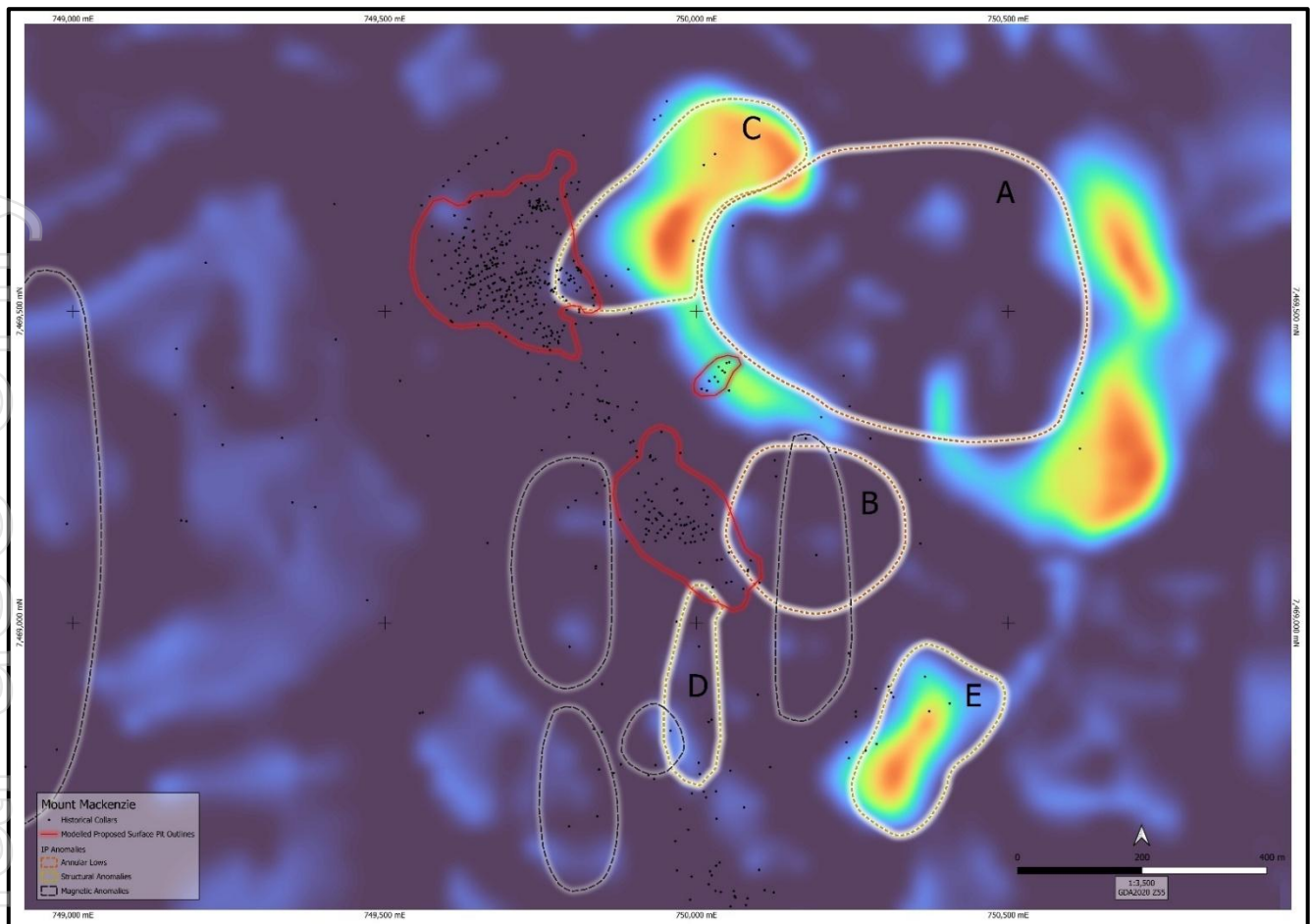
Figure 5: 50m depth slice chargeability showing Target A annular low and Targets C and E structural highs.
