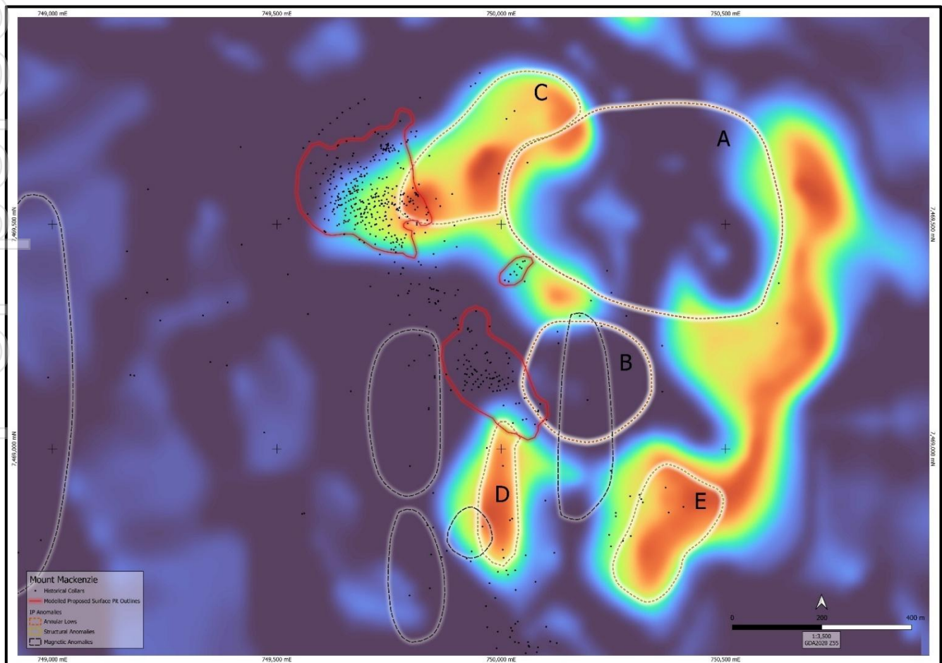
Figure 6: 100m depth slice chargeability showing Target B annular development and Target C.
