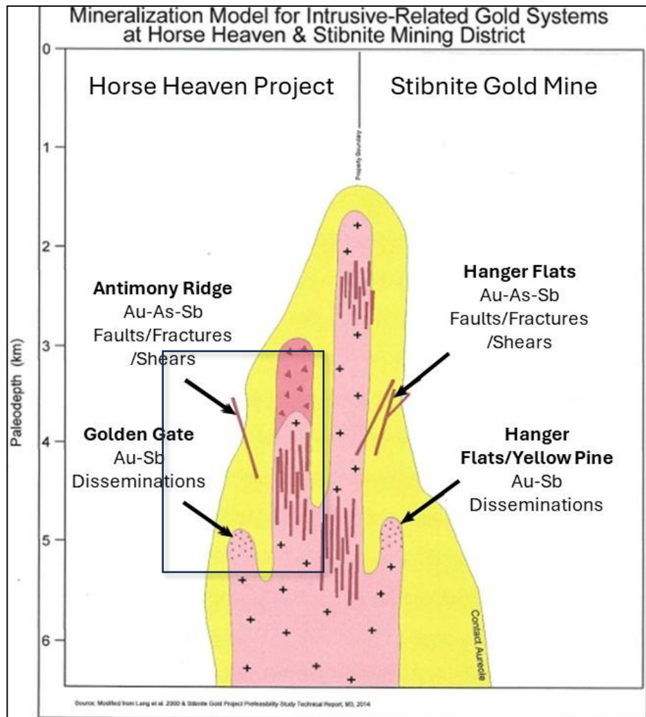
Figure 6: Schematic IRGS cross section showing the relative positions of the Stibnite Mining District Hanger Flats and Yellow Pine deposits (Right half) and the Antimony Ridge and Golden Gate prospects (Left half). This cross section is modified from Lang et al 2000. This image first appeared in the RML announcement of 11 June 2025.
