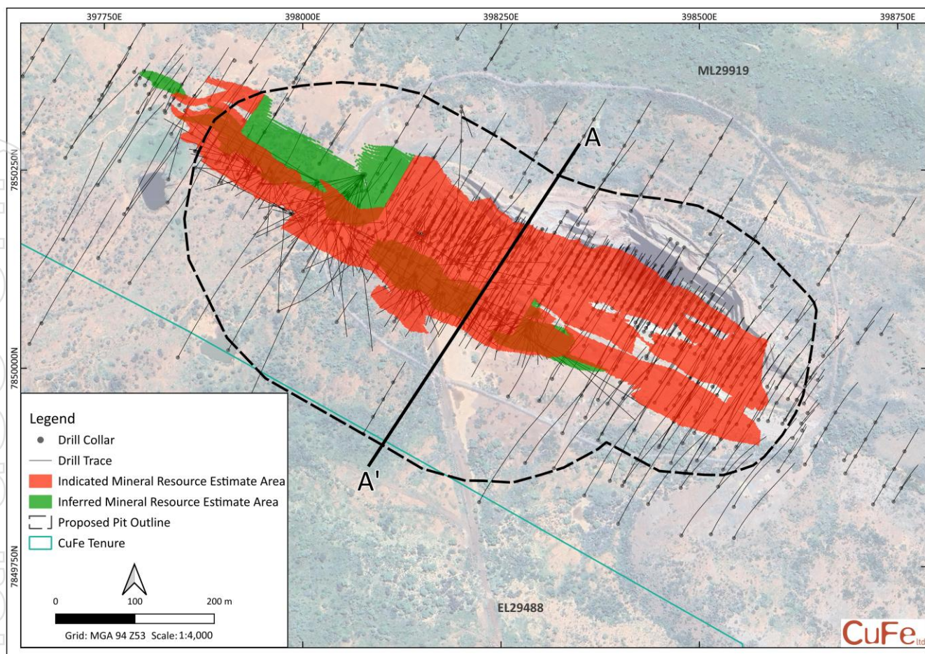
Figure 2: The Orlando Deposit and drill hole locations in plan view with resource category shown.
