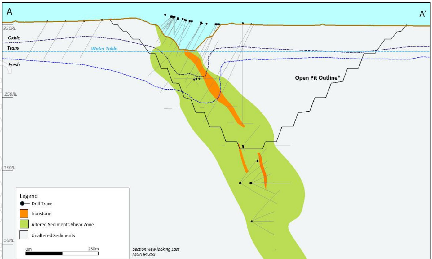
Figure 4: Cross section of the geological model used for the March 2026 Orlando MRE update. Section A-A1 line is shown in Figure 2.
