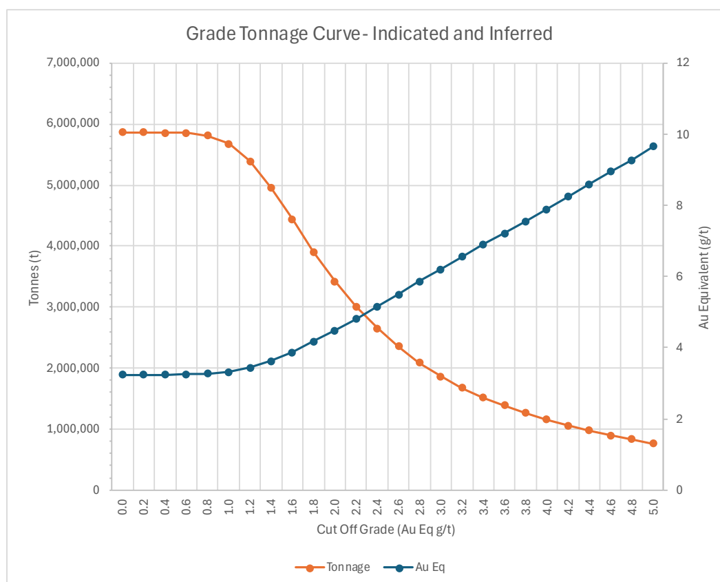
Figure 5: 2026 Orlando Mineral Resource Grade Tonnage Curve
