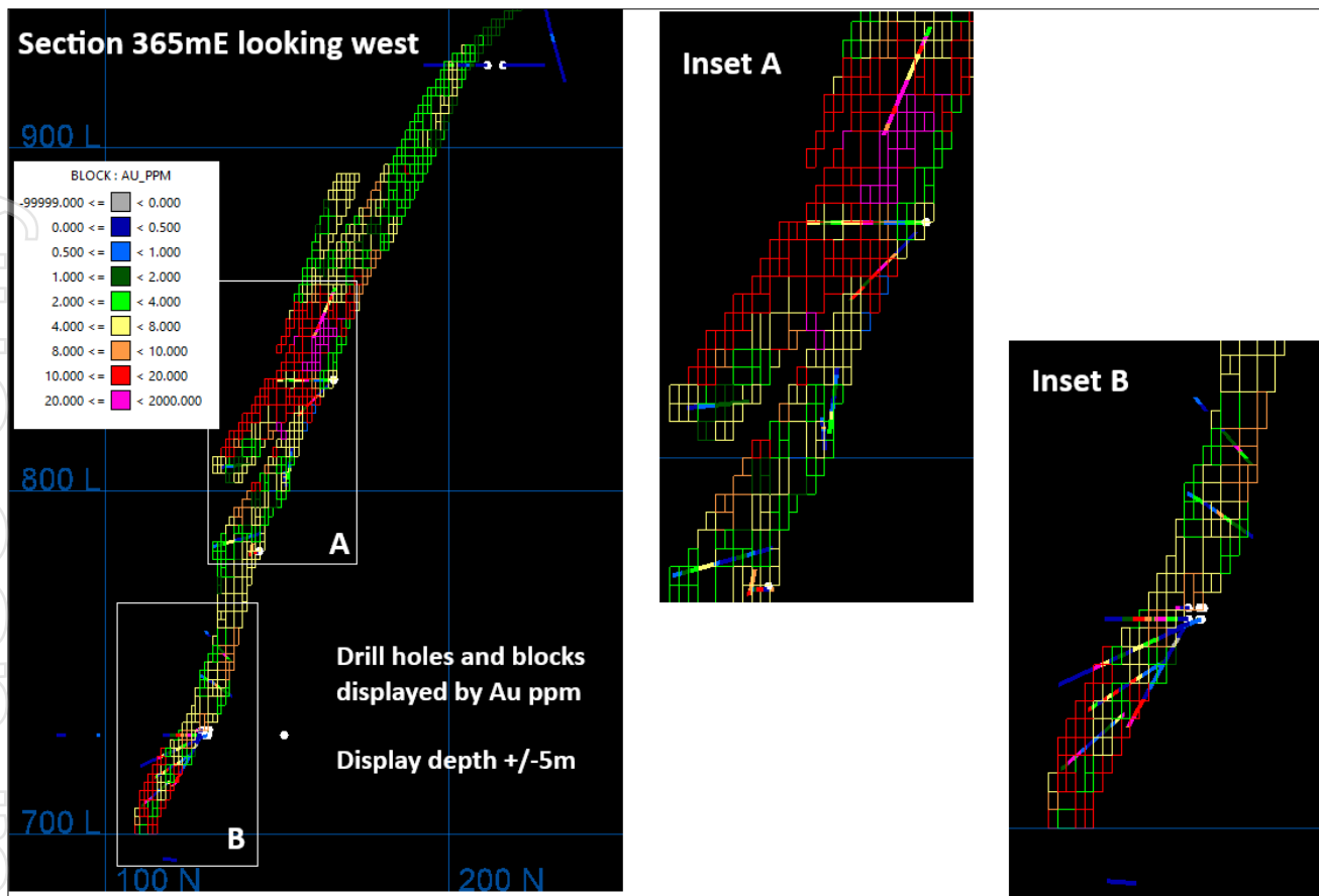
Figure 6: Gold grades in drillholes versus estimated block grades.
