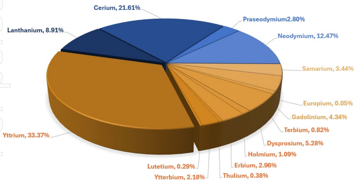
Figure 2: Pie Chart displaying average REO distribution for all Lodestar Resources samples with TREO >1%
