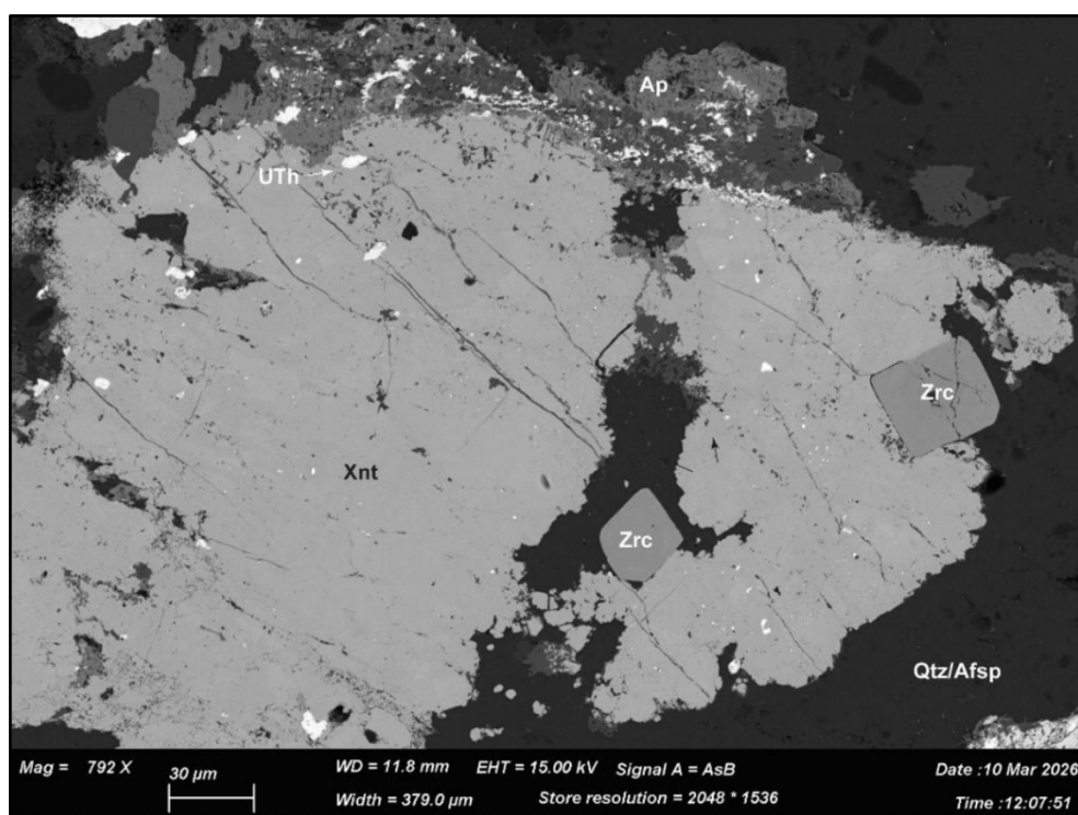
Figure 4: SEM image of sample CA50, Xenotime & Zircon – grey, Quartz/Feldspar - Black
