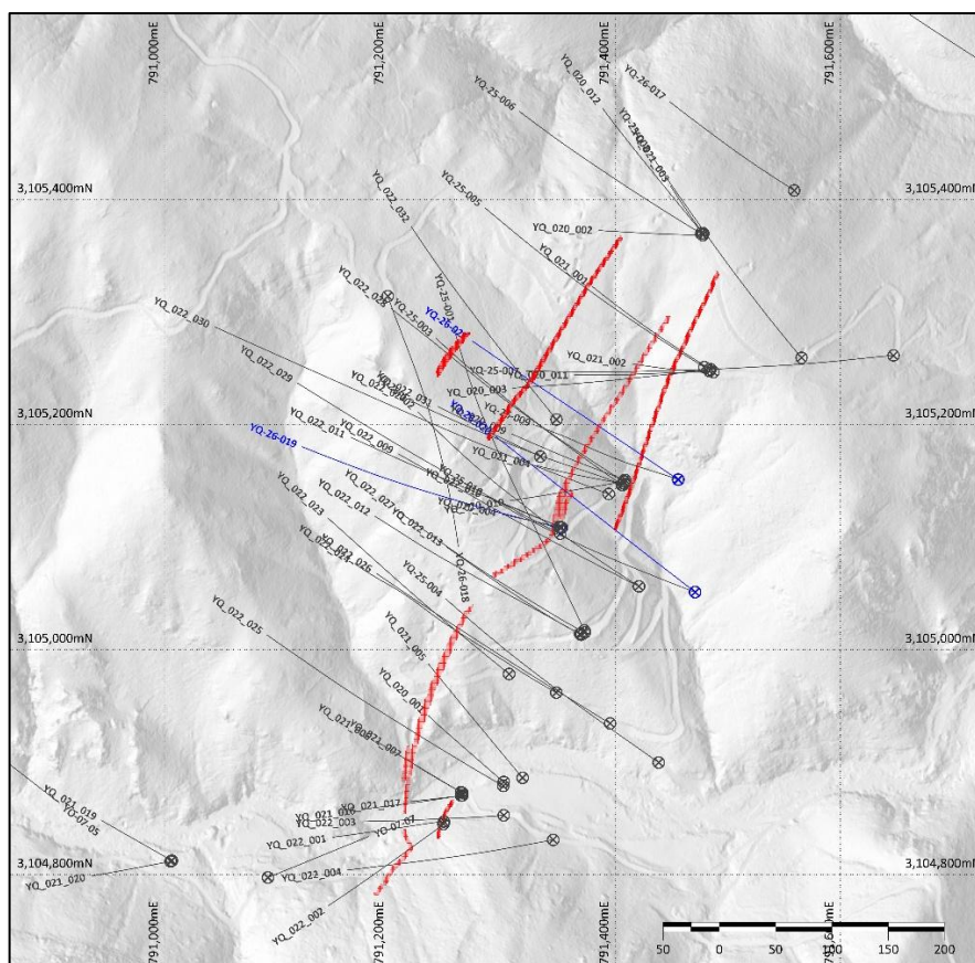
Figure 4. Plan of the Pertencia area at Yoquivo showing existing drill holes 2 (black) and new drill holes (blue) over recently collected high-resolution LiDAR topography data. A projection of the existing Foreign Estimate 2,3 at 1,960RL is also shown in red.
