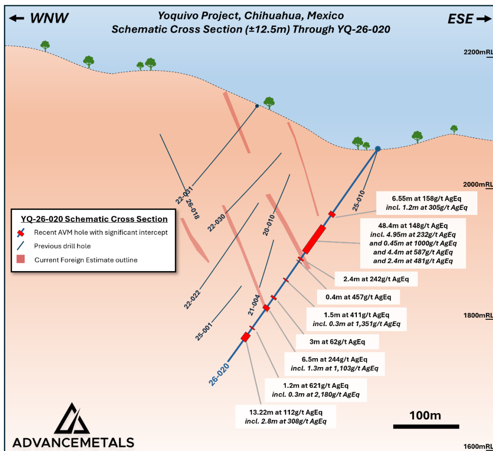
Figure 3. Schematic cross section (±12.5m, looking north-northeast) through hole YQ-26-020 showing previous drilling 2 and an approximate outline of the existing Foreign Estimate 2,3 .
