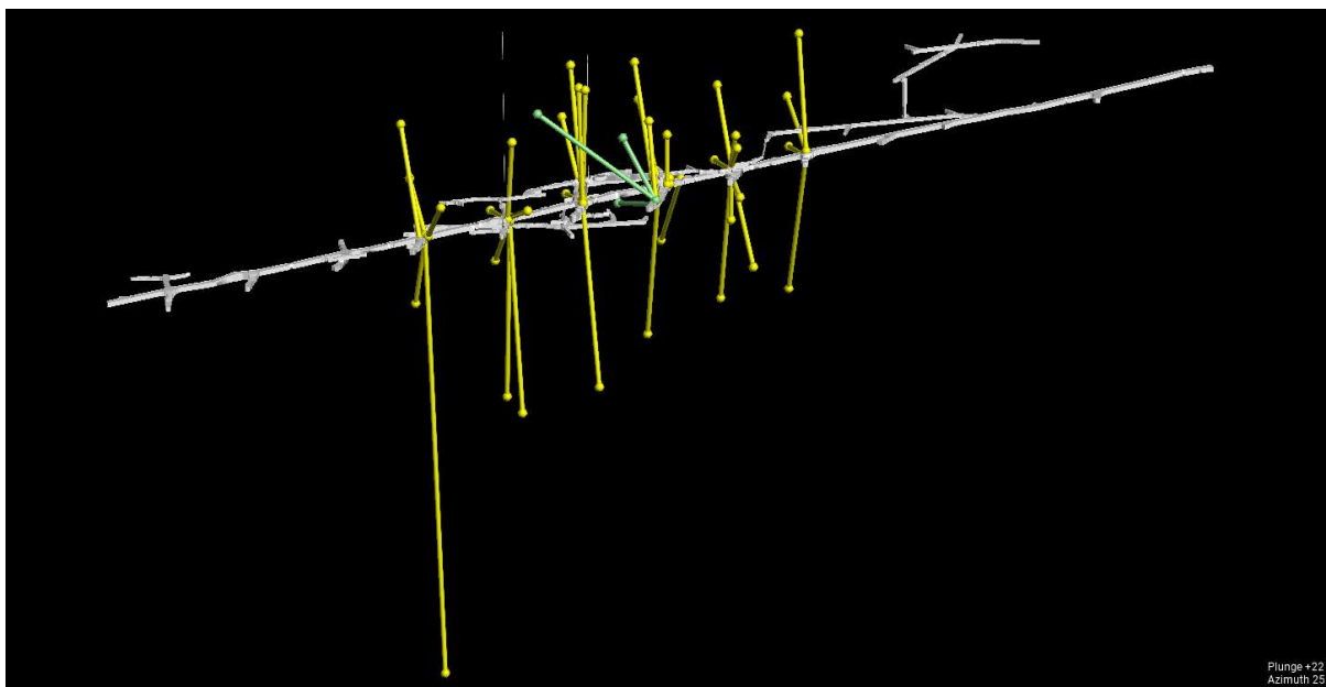
Figure 3: Oblique view (looking WNW from slightly above) of Lincoln Gold Project showing location of Stringbean Alley Decline, and location of drilled sections from respective crosscuts XC3-XC8 (viewed from Right to Left). Oblique series of holes from XC5E denoted in green.
