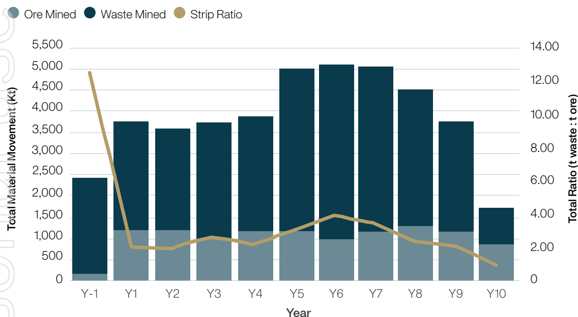
Figure 50: Annual total material movement by ore and waste.
