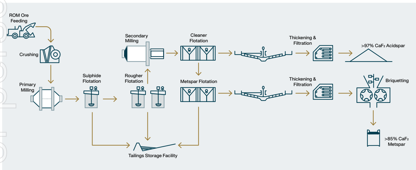
Figure 55: Speewah Fluorite Project process flowsheet.
