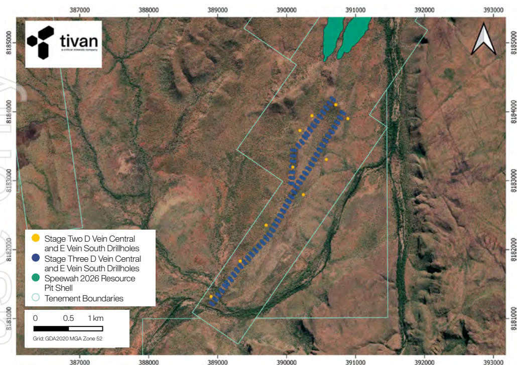
Figure 39: Stage Three D-Vein Central and E Vein South planned exploration drilling, with Stage Two wide spaced drilling shown for spatial context.
