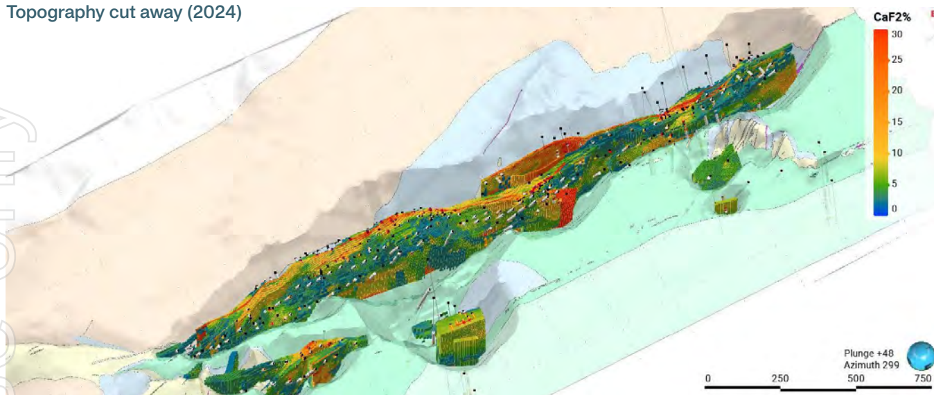
Figure 20: 2024 Resource Estimate Block model and drilling within the constraining pit shell coloured by CaF 2 %.
