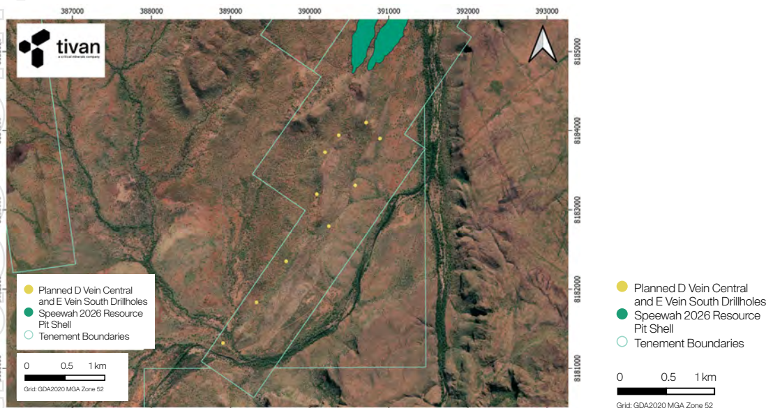
Figure 36: Planned wide spaced drilling at the D-Vein Central and E-Vein South Exploration Targets.
