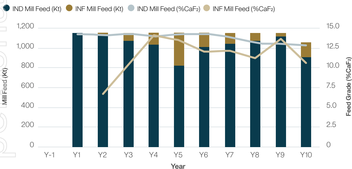
Figure 52: Annual mill feed by resource classification.
