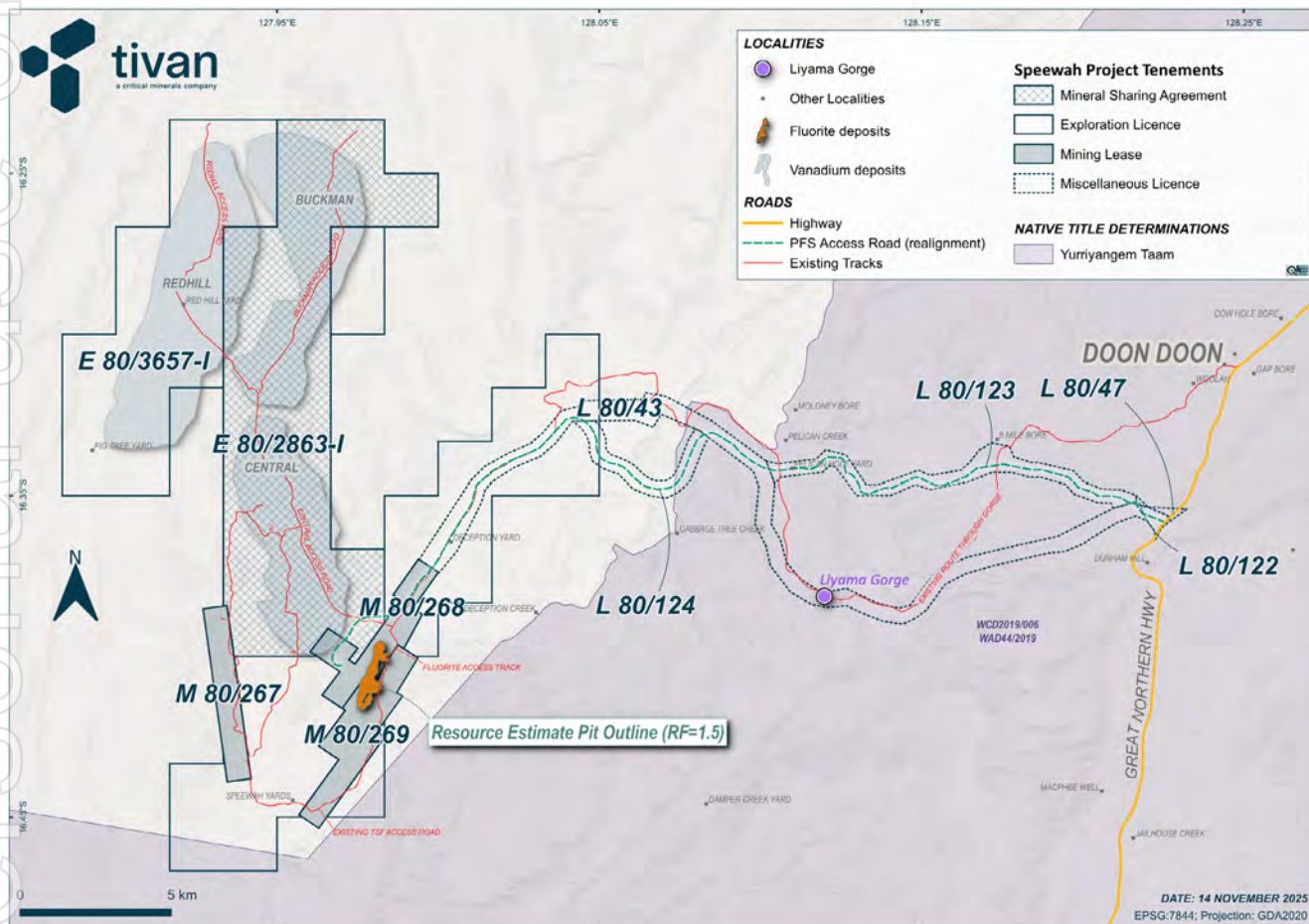
Figure 15: Speewah Fluorite Project with tenement and exploration track overlay.
