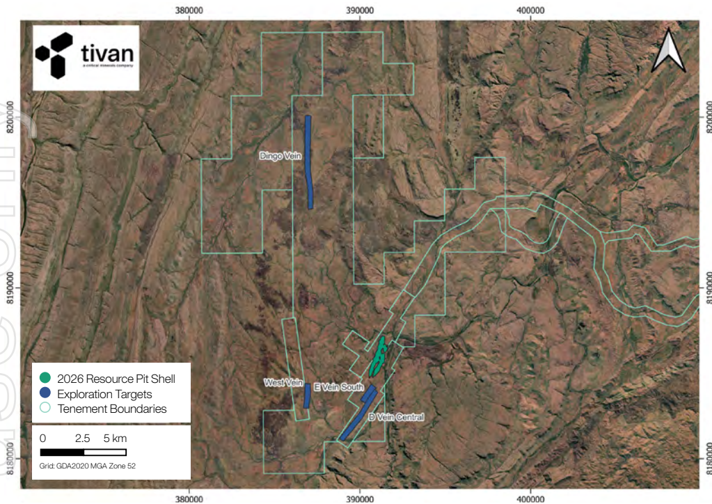
Figure 26: 2024 Exploration targets remaining after 2025 drill campaign completed by Tivan.
