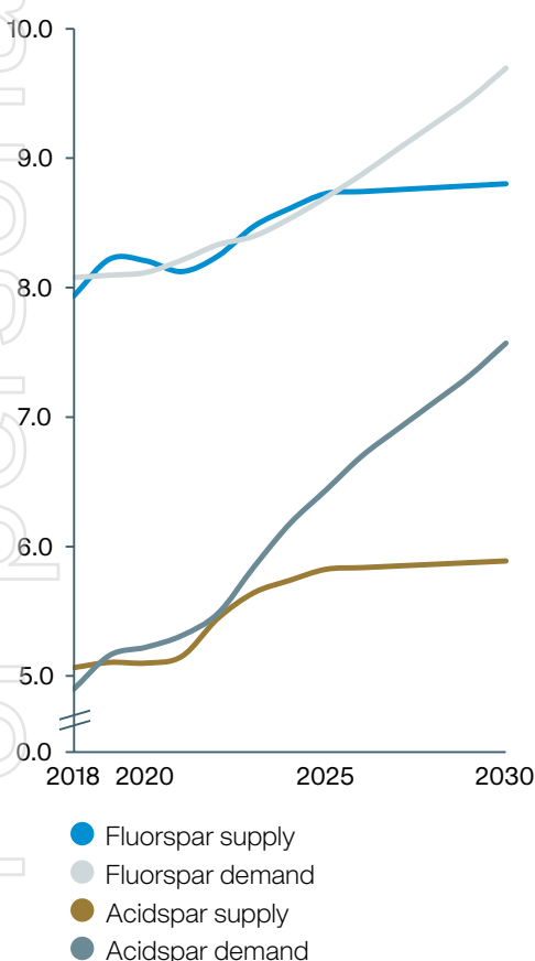
Figure 5: Fluorspar Supply and demand; upstream and midstream; actual and forecast.
