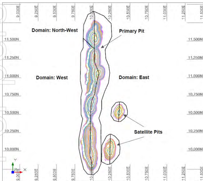
Figure 48: Pit design geotechnical domains.
