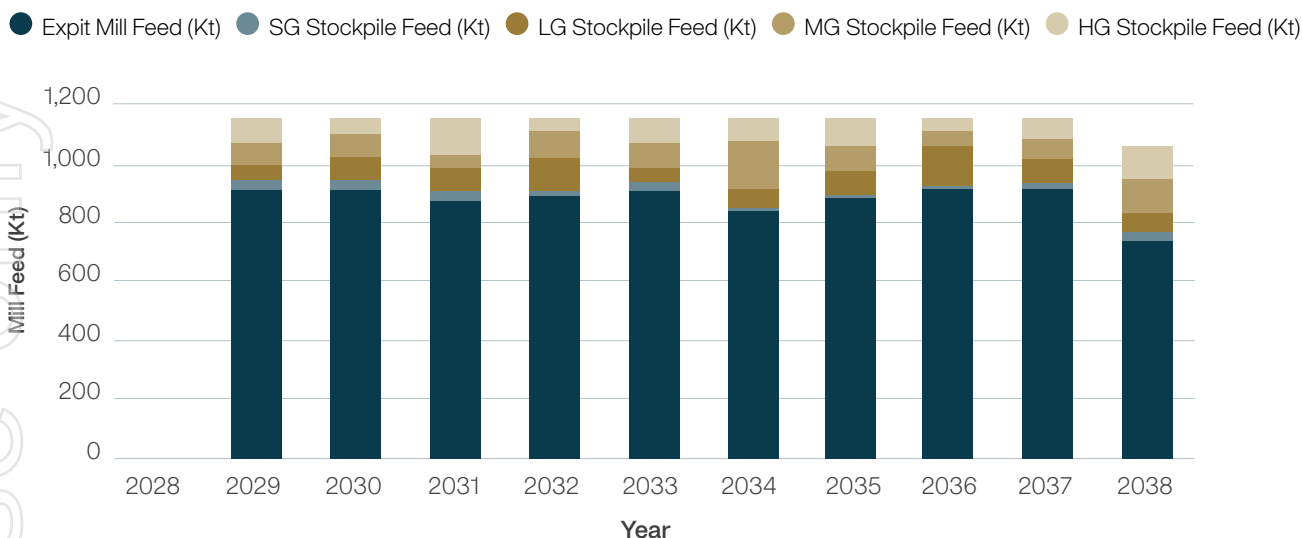
Figure 53: Annual mill feed by source location.
