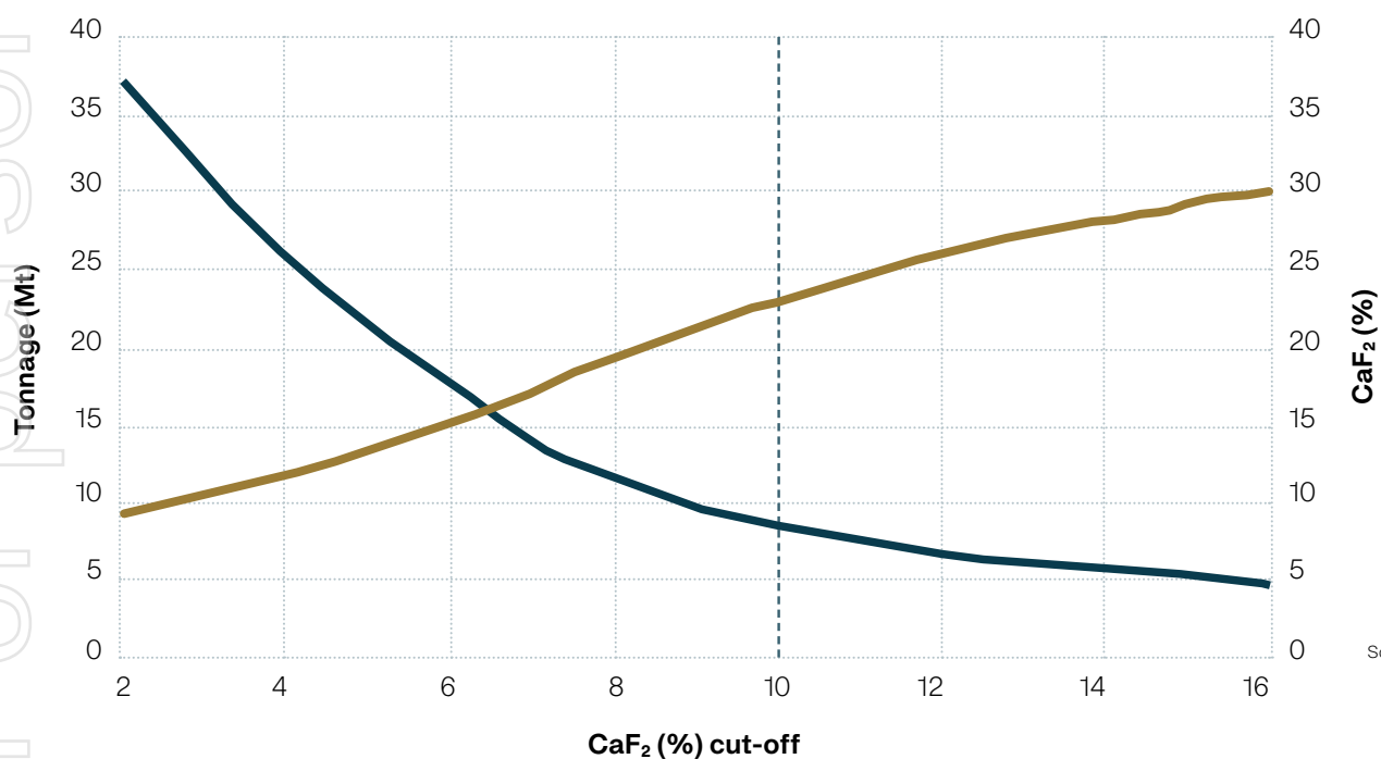
Figure 21: Grade and tonnage curves – 2024 Mineral Resource material.
