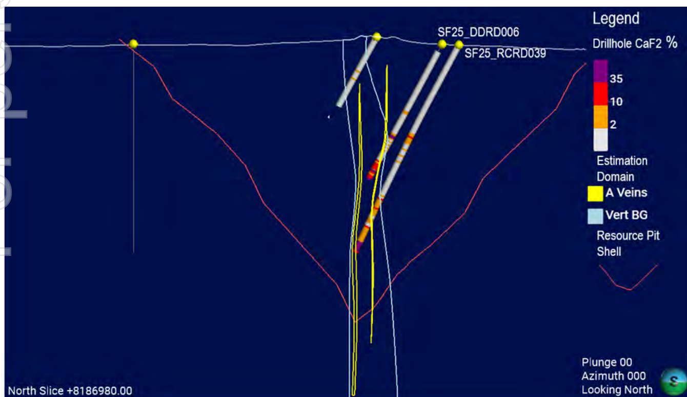
Figure 29: Cross section of A-Vein North extension drilling from Speewah geological model.
