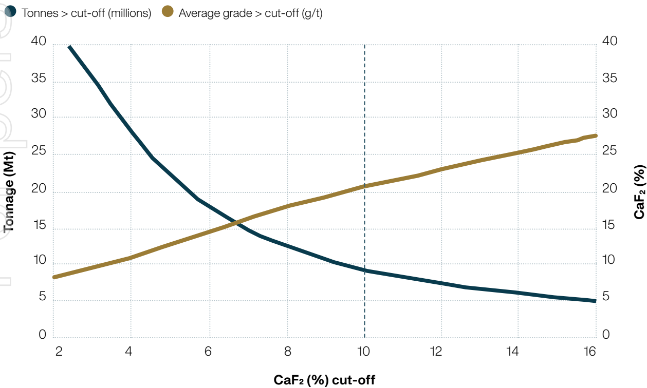
Figure 23: Grade and tonnage curves – 2026 Mineral Resource material.
