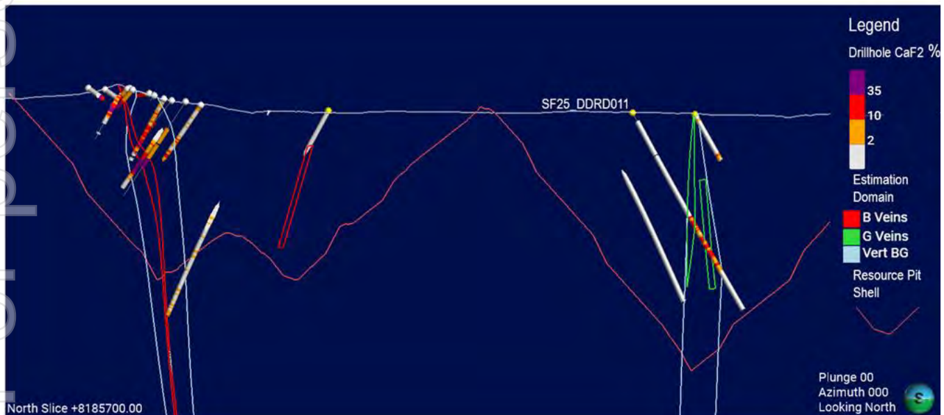
Figure 31: Cross section of G-Vein Link extension drilling from Speewah geological model.
