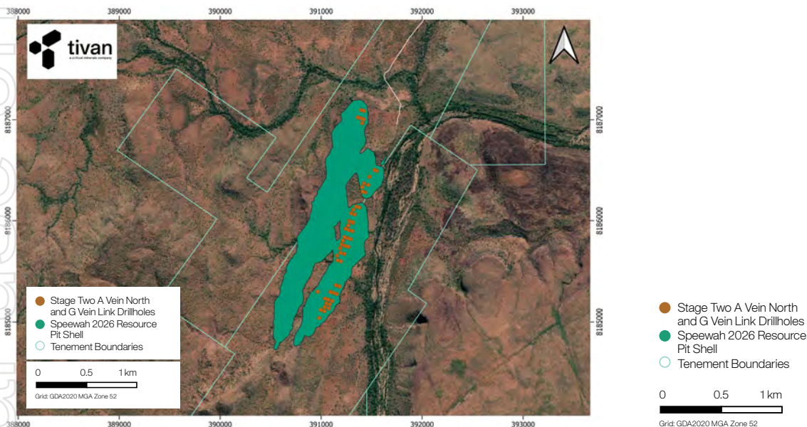
Figure 32: Stage Two A-Vein North and G-Vein Link indicated infill drilling.
