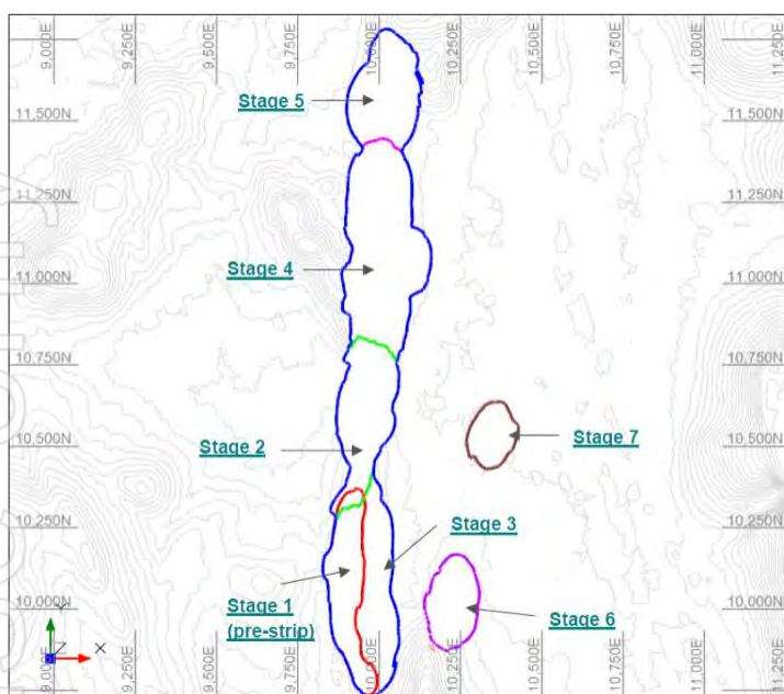
Figure 47: Strategic pit staging – plan view of pit stages.
