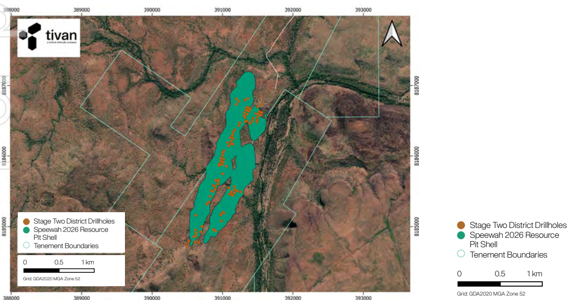
Figure 33: Stage Two Central Zone Indicated Infill drilling.
