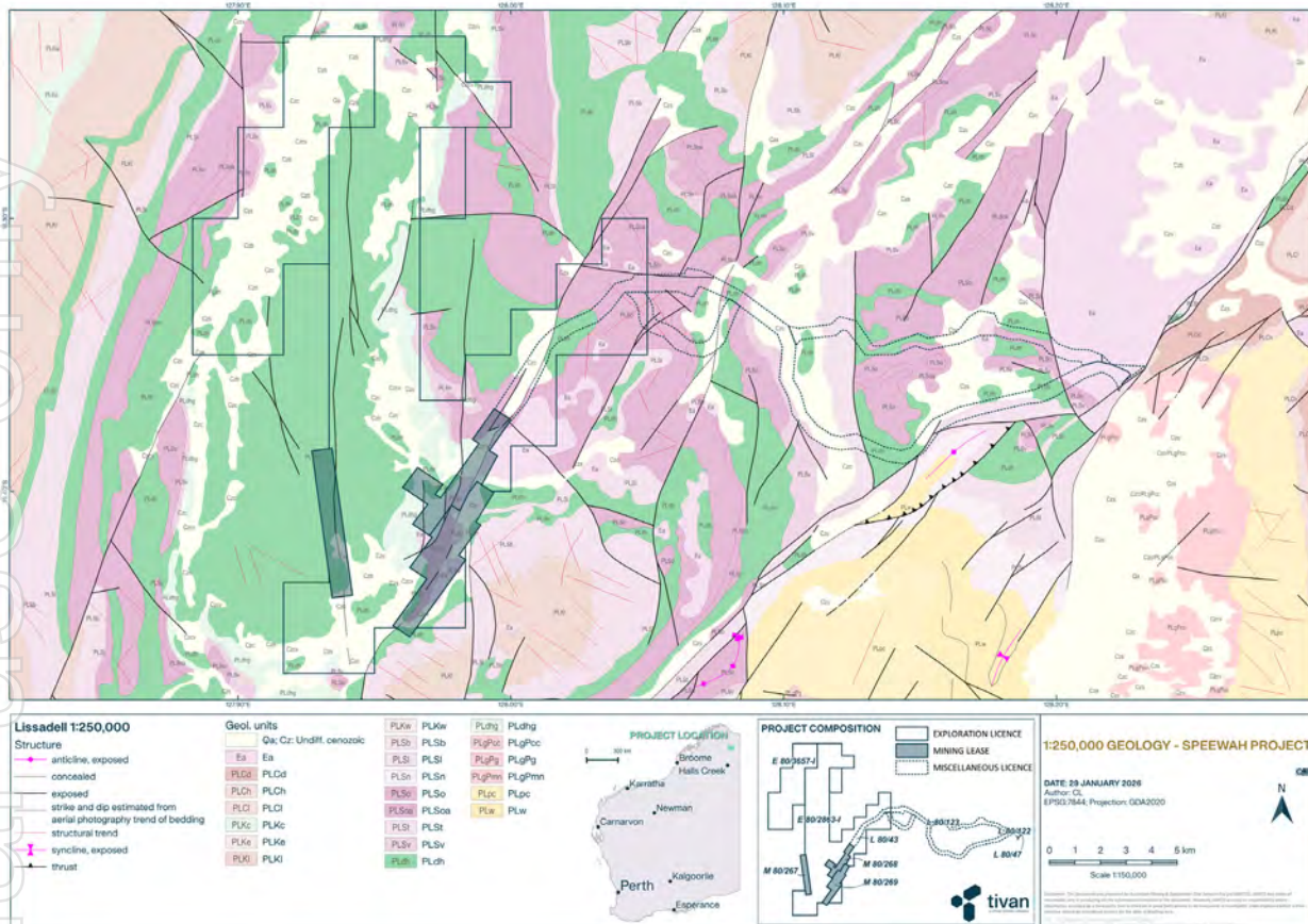
Figure 17: Geology of Speewah.
