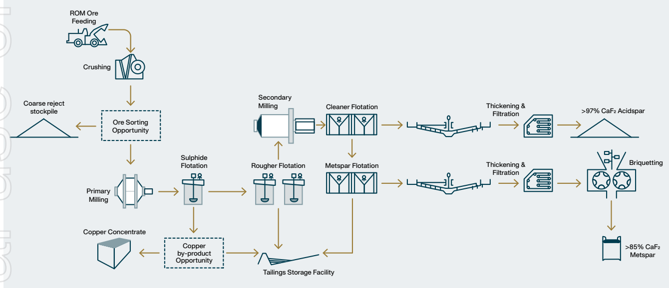
Figure 59: Speewah Fluorite Project process flowsheet with potential ore sorting and copper concentrate by-product.
