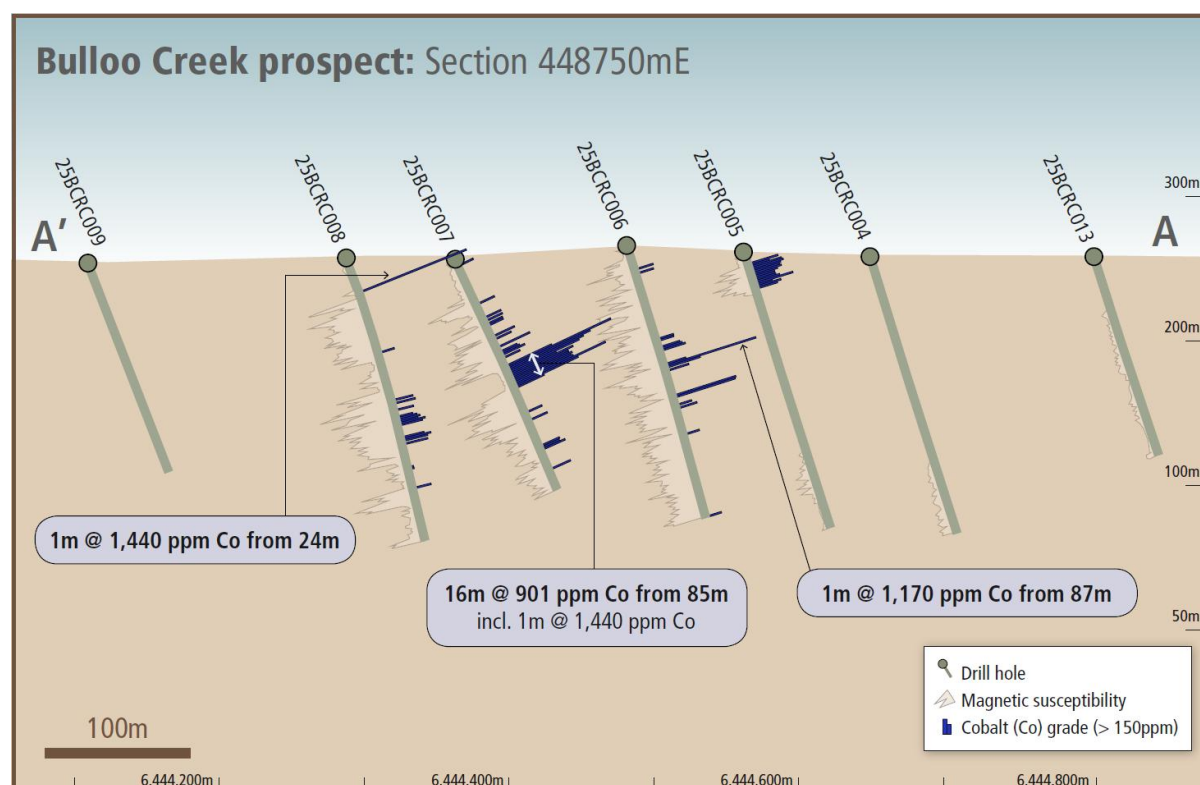
Figure 2. Eastern Anomaly zone sub-surface section along 448750E focused on cobalt assay results and magnetic susceptibility.
