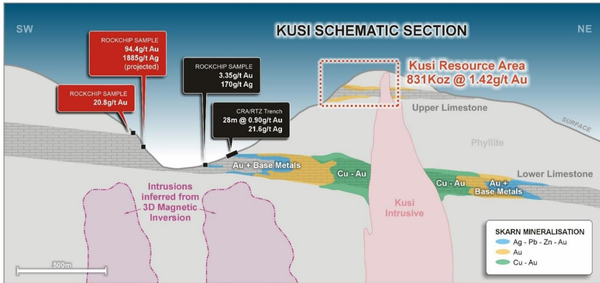
Figure 3 - Conceptual cross-section at Kusi showing intrusions into limestone units which host mineralisation.
