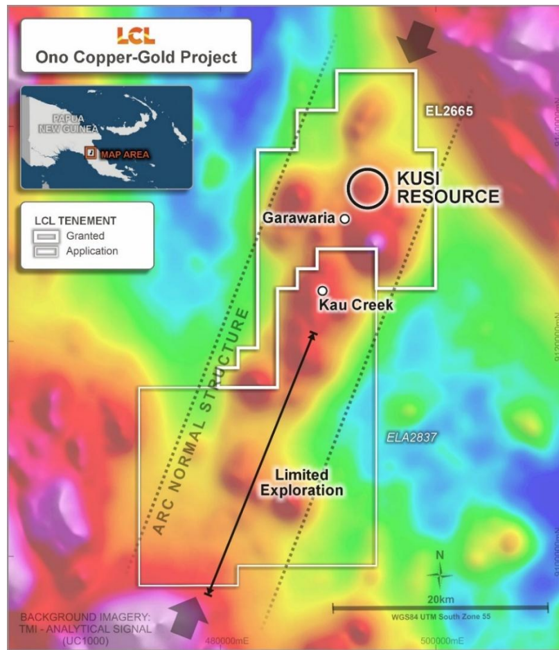
Figure 2 - Total Magnetic Intensity image (Analytical Signal) showing cross-arc structure and associated magnetic intrusive bodies.
