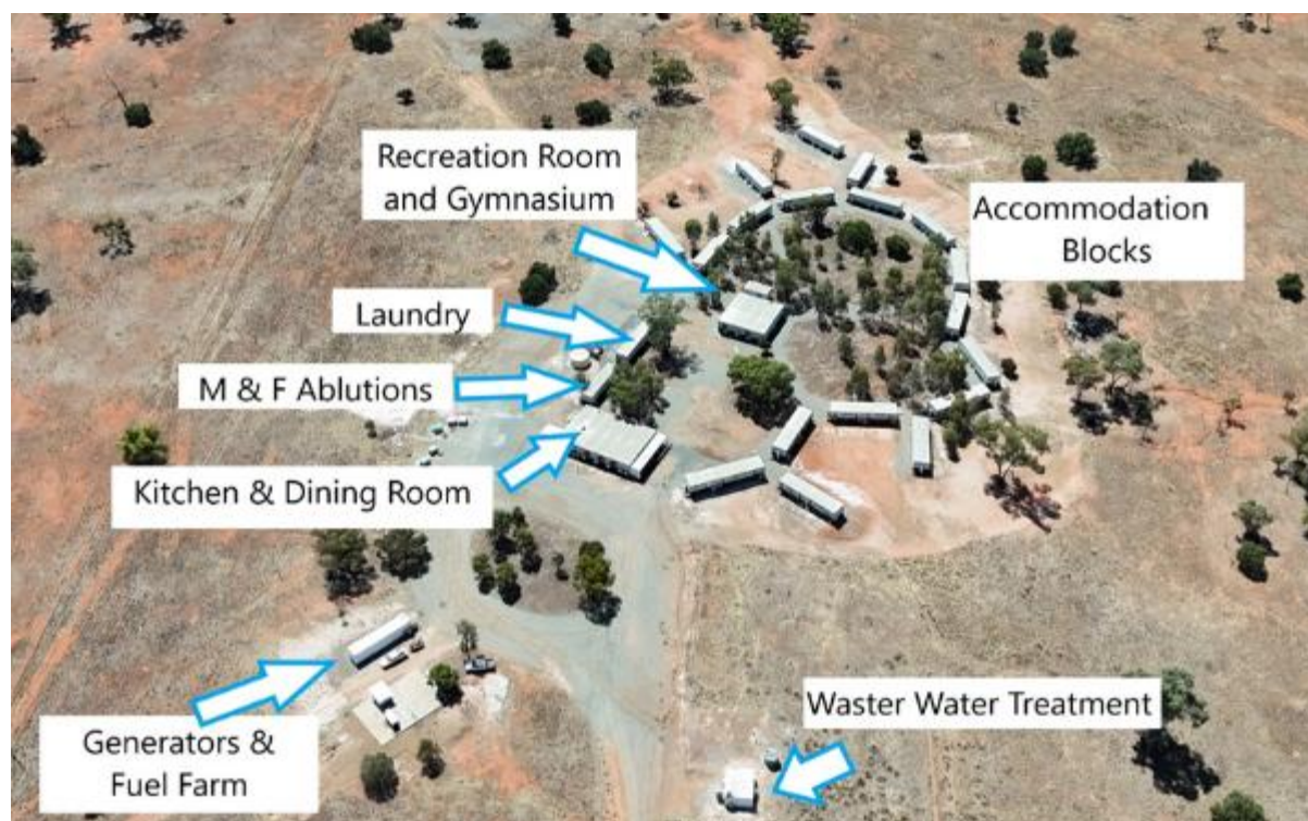
Figure A20: Layout of the existing accommodation camp
