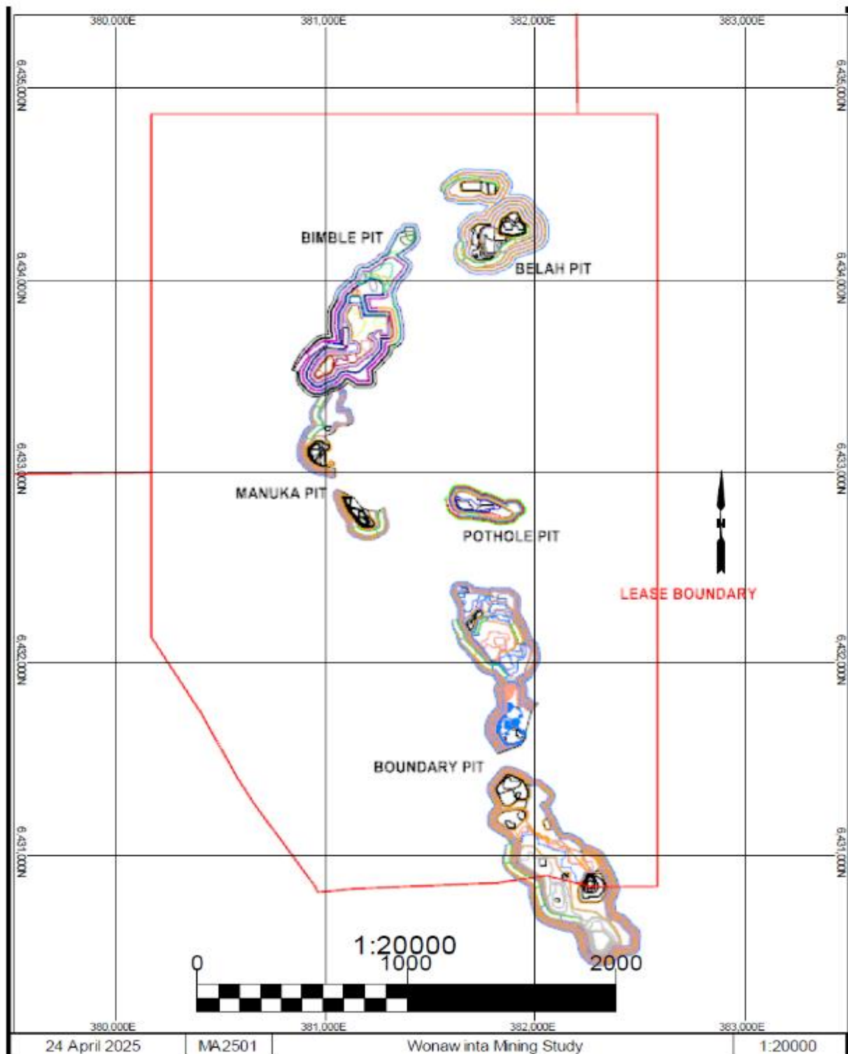
Figure A8: Life of Mine Pit Designs
