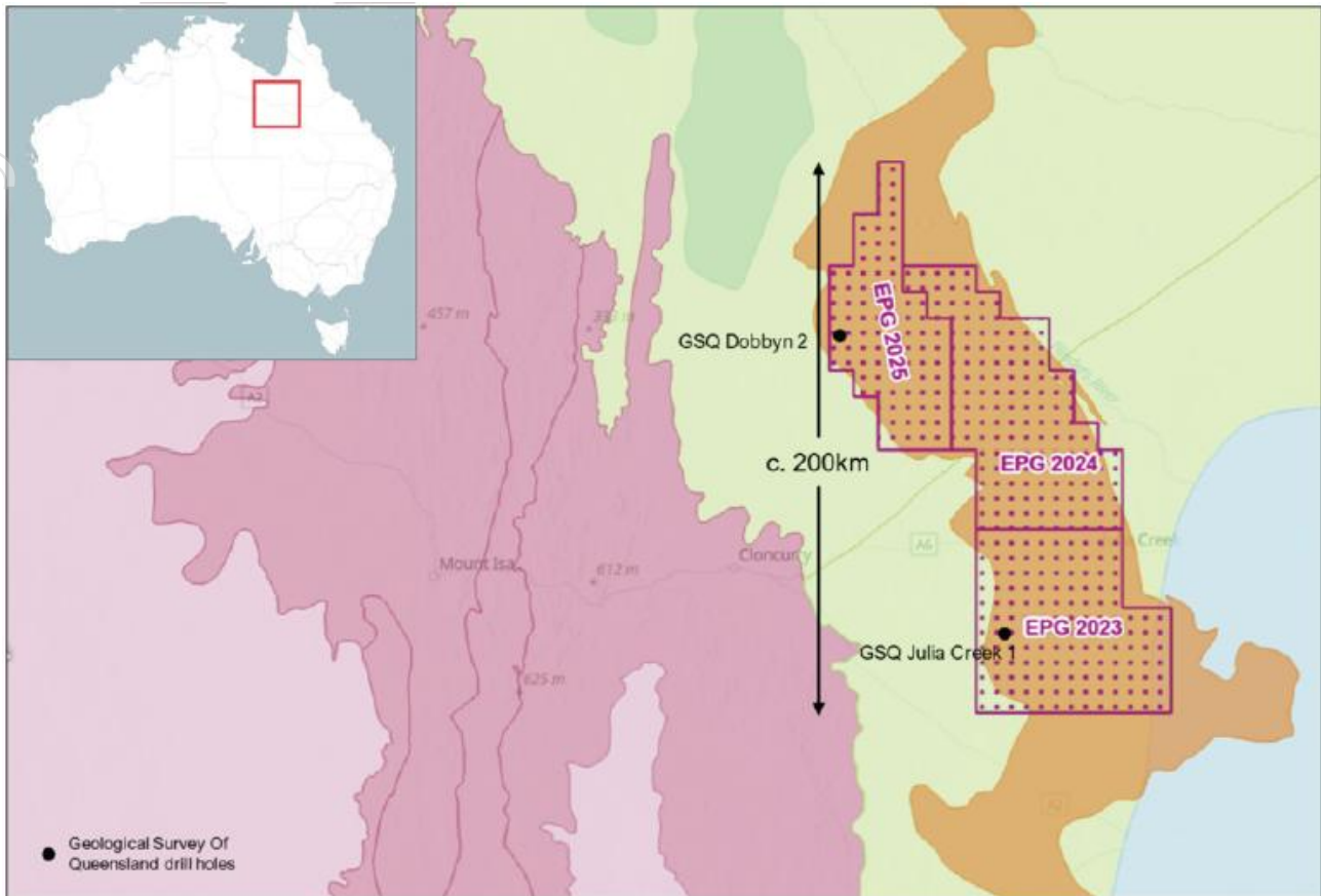
Figure 1: Millungera Basin location (in brown) to the east of the Mt Isa Inlier (in red) and EPG permit areas, north-west Queensland. Inset shows position within Australia.
