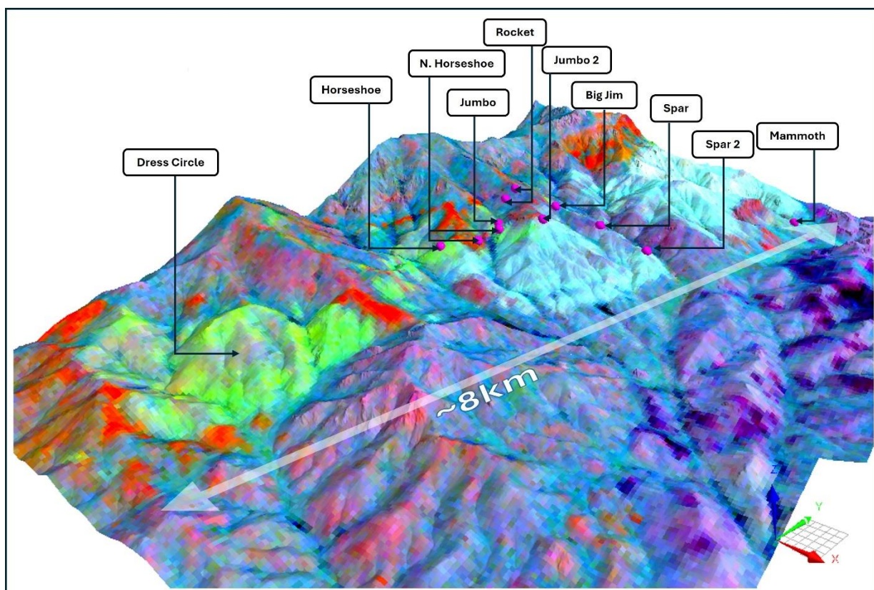
Figure 1 Frontispiece: EnMap alteration index draped on elevation model with fluorspar occurrences. View NW. (refer Figure 2 for descriptions)
