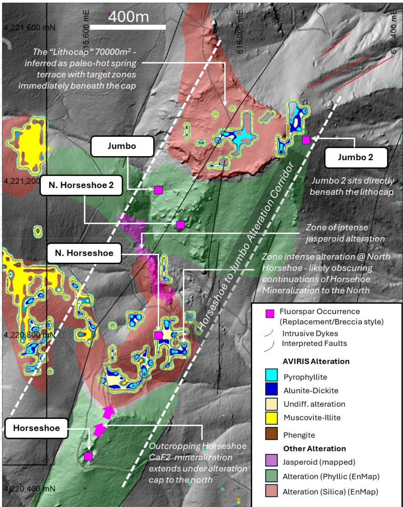
Figure 3 AVIRIS hyperspectral alteration map showing the potential continuations of the Horseshoe Corridor.
