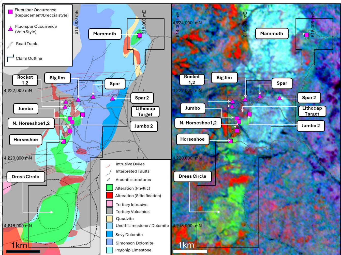
Figure 2. (Left) Alteration interpretation overlying geological interpretation with mineral occurrences and target zones. (Right) The processed alteration map from EnMap spectral satellite imagery: green shades indicate phyllic alteration; red shades indicate silica alteration or silica rocks; pale blue indicates unaltered carbonate rocks
