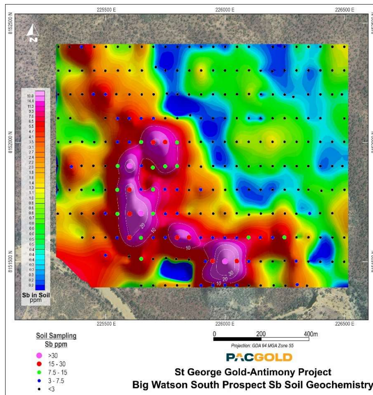
Figure 4: Big Watson South Prospect – geochemical soil sample assay results – Antimony
