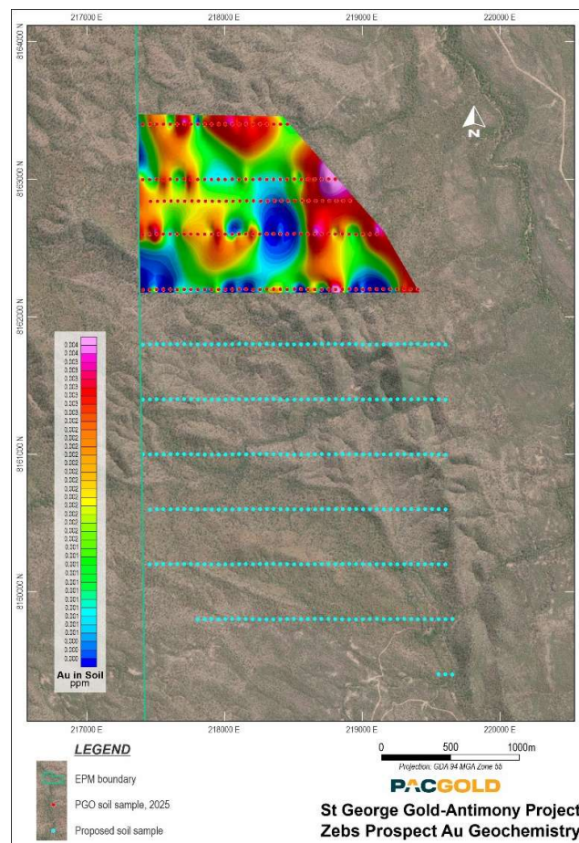
Figure 7: Zebs Prospect – geochemical soil sample assay results – Gold. Note blue dots are proposed sample locations.
