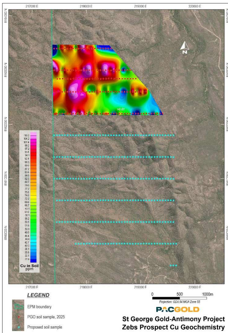
Figure 8: Zebs Prospect – geochemical soil sample assay results – Copper . Note blue dots are proposed sample locations.
