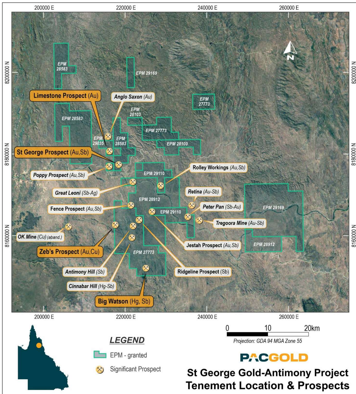
Figure 1: St George Project tenement package map with known historical gold and antimony occurrences, and priority prospect
