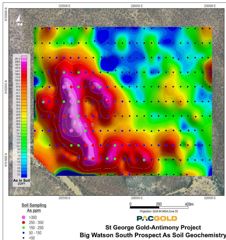
Figure 5: Big Watson South Prospect – geochemical soil sample assay results – Arsenic
