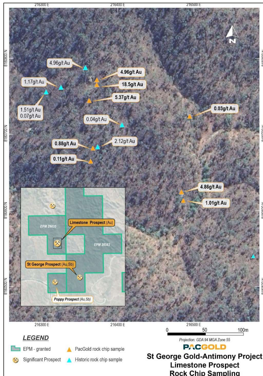
Figure 6: Limestone Prospect – High Grade gold rock chip sample assay results
