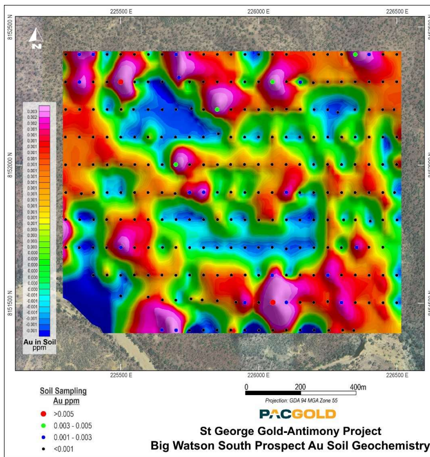
Figure 3: Big Watson South Prospect – geochemical soil sample assay results – Gold
