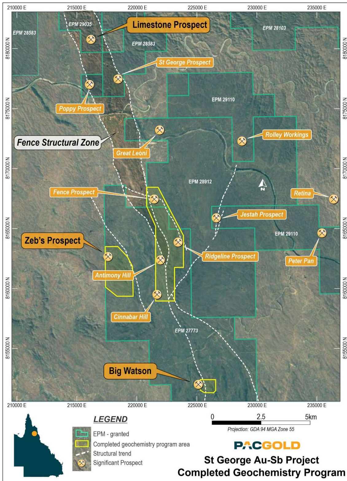
Figure 2: Fence Structural Zone, with location of Big Watson South, Limestone and Zebs Prospects
