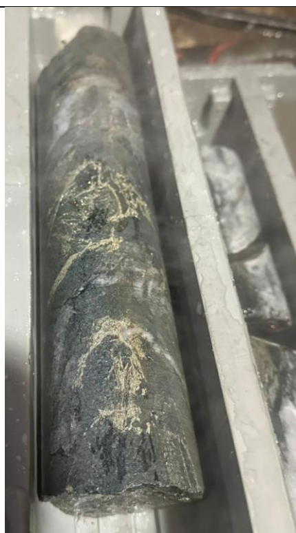
Figure 3 – Close-up of sulphide mineralisation
