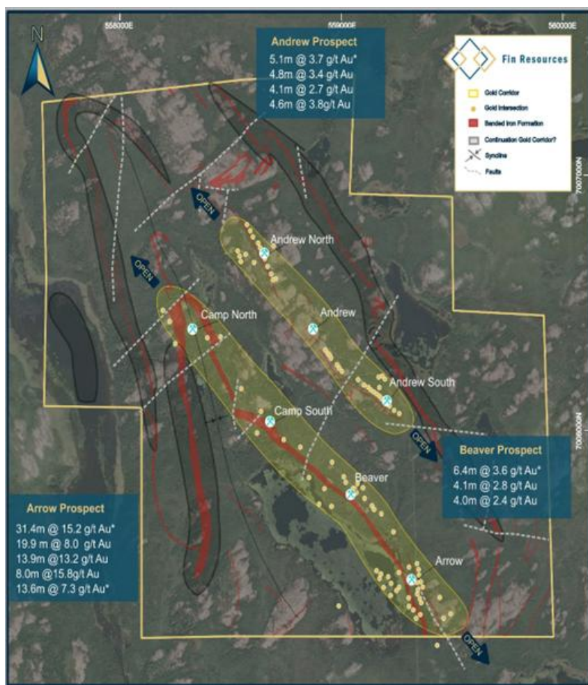
Figure 4 - Cabin Lake Gold Project: Historical Drillhole Locations and Prior Sampling Results
