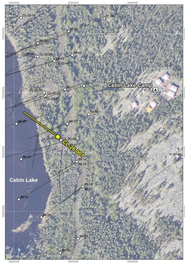
Cabin Lake – Plan View – Drillhole CL-26-001
