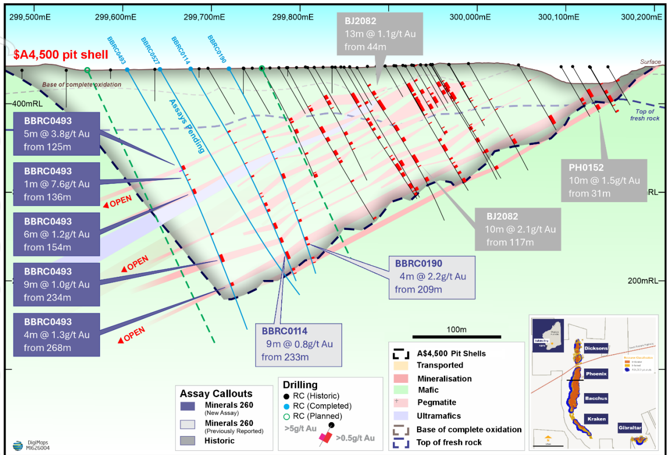
Figure 4 - Section 6567980N showing high-grade mineralisation at Phoenix in drill hole BBRC0493 internal to the MRE pit shell (new results in purple boxes)
