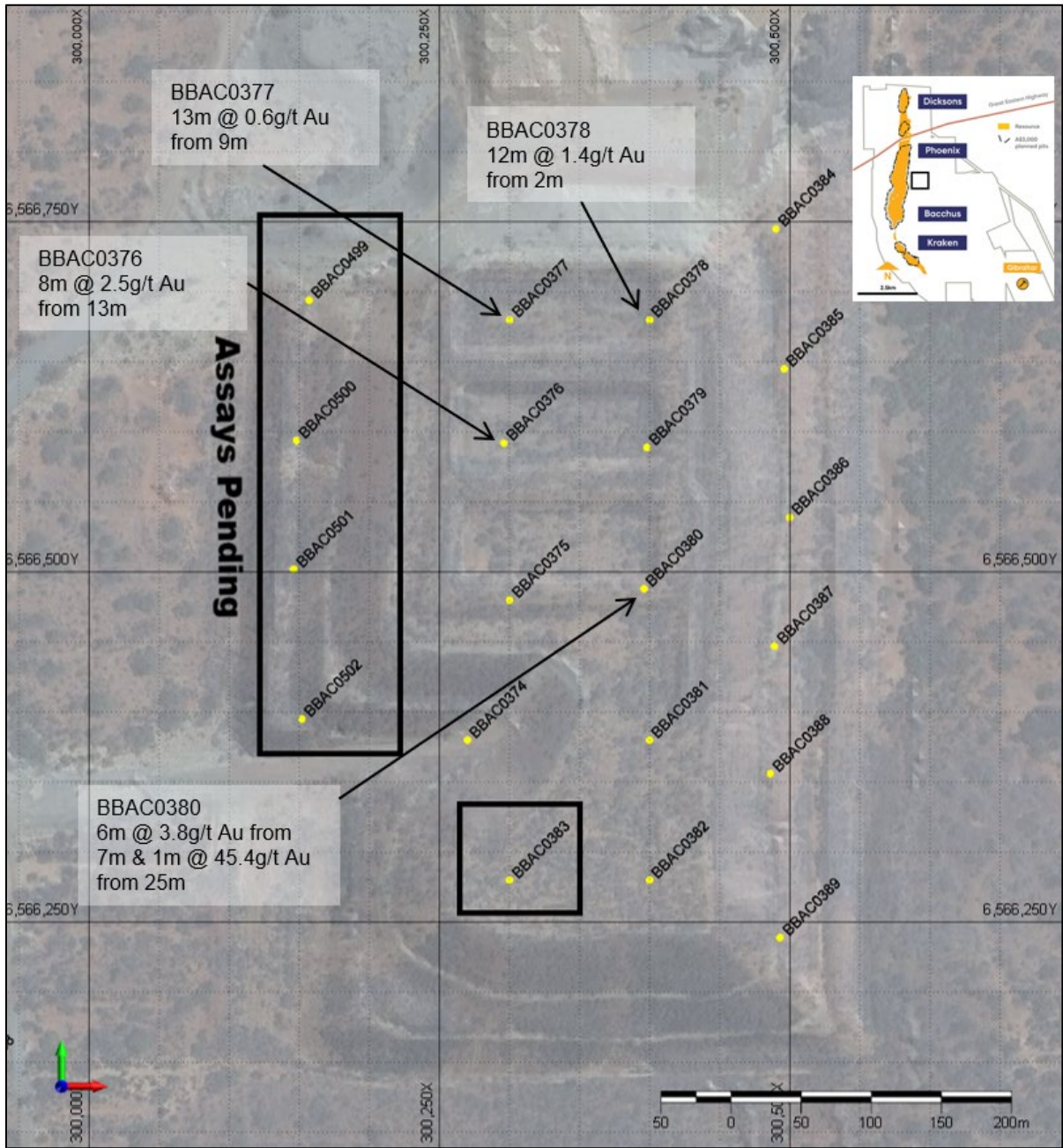
Figure 5 - Bacchus Waste Rock Dump East showing drill collar locations with significant intercepts
