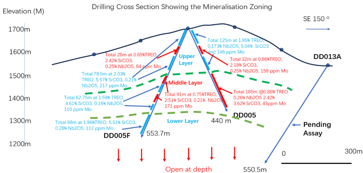
Figure 2: Drilling Cross Section illustrating mineralization zoning across the NW Line with latest hole being DD005F
