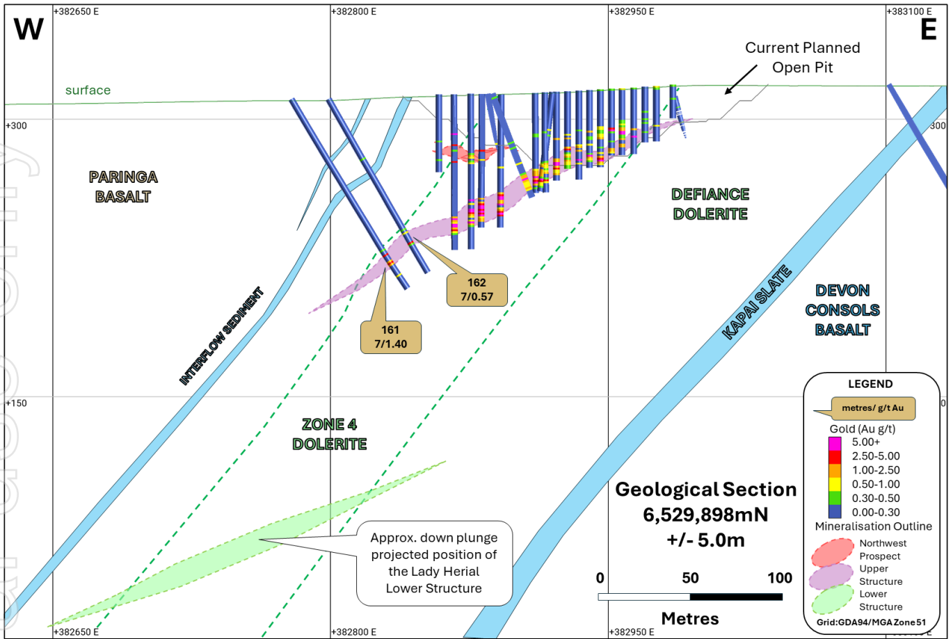
Figure 4: Cross section 6,529,898mN - view of the Lady Herial area showing today's and prior results (unlabelled).
