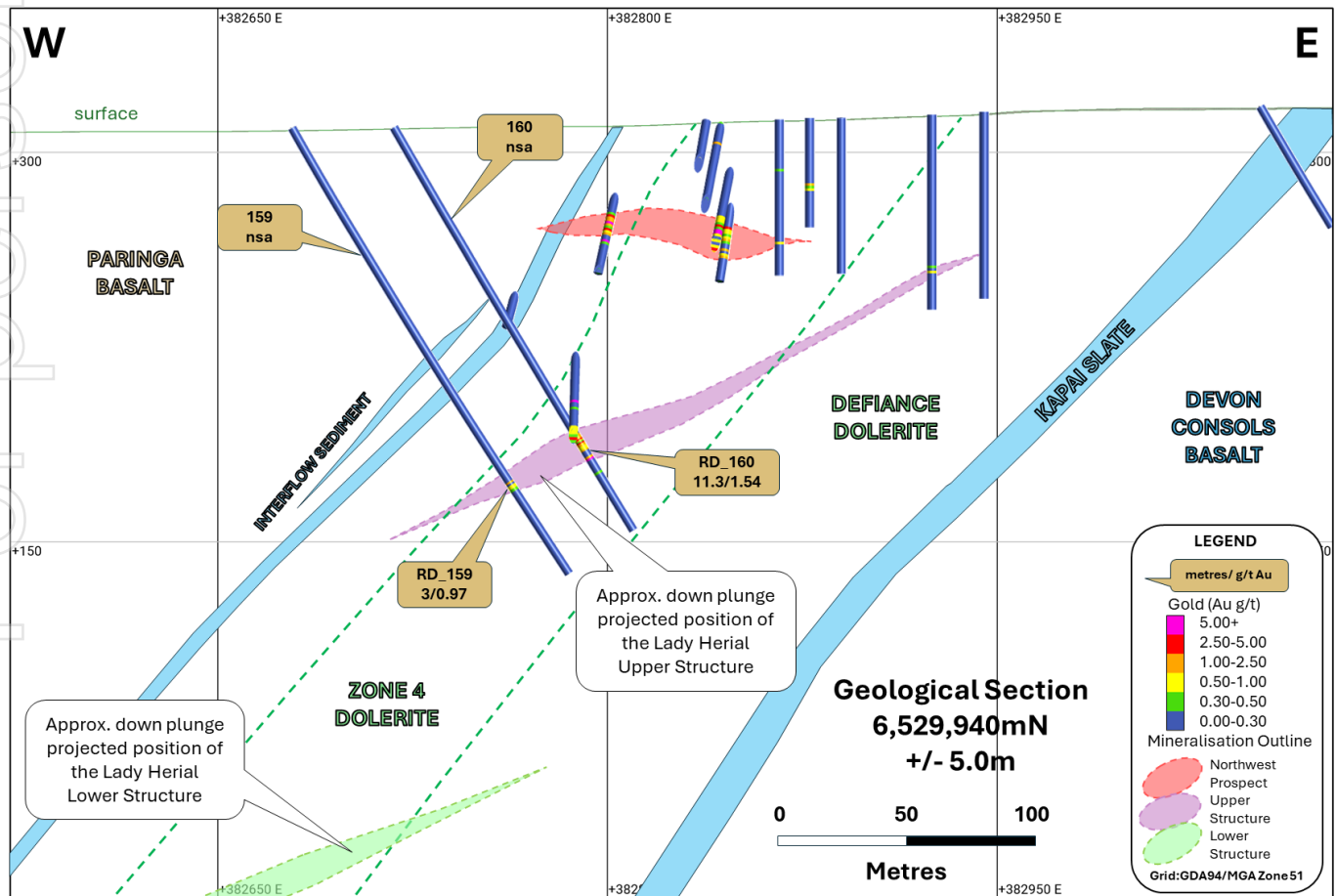
Figure 5: Cross section 6,529,940mN view of the Lady Herial area showing today's and prior results (unlabelled).
