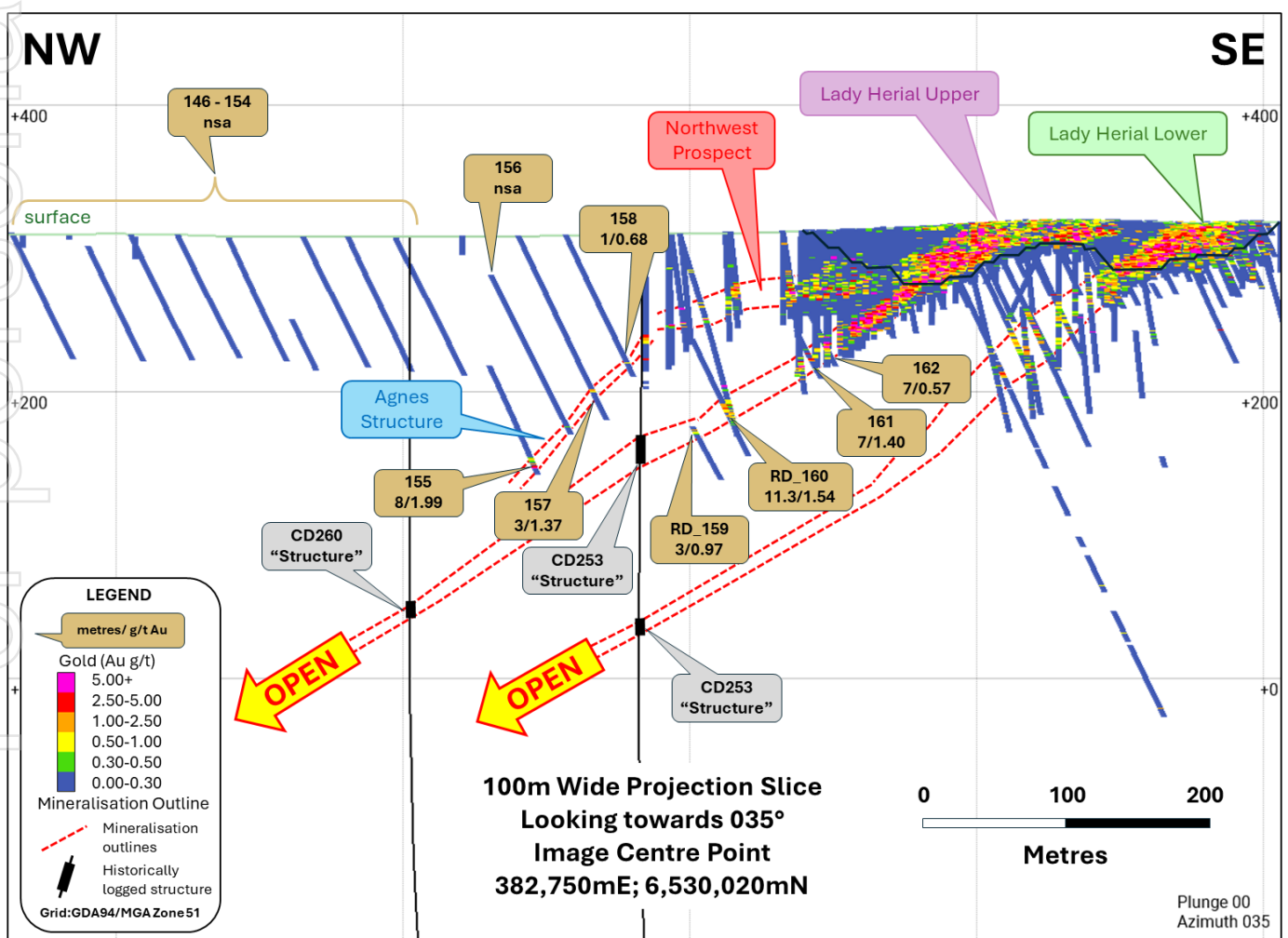
Figure 3: Long sectional view of the broader Lady Herial area showing today's results, the historical WMC holes (grey callouts) and the relative location of the various mineralised structures.
