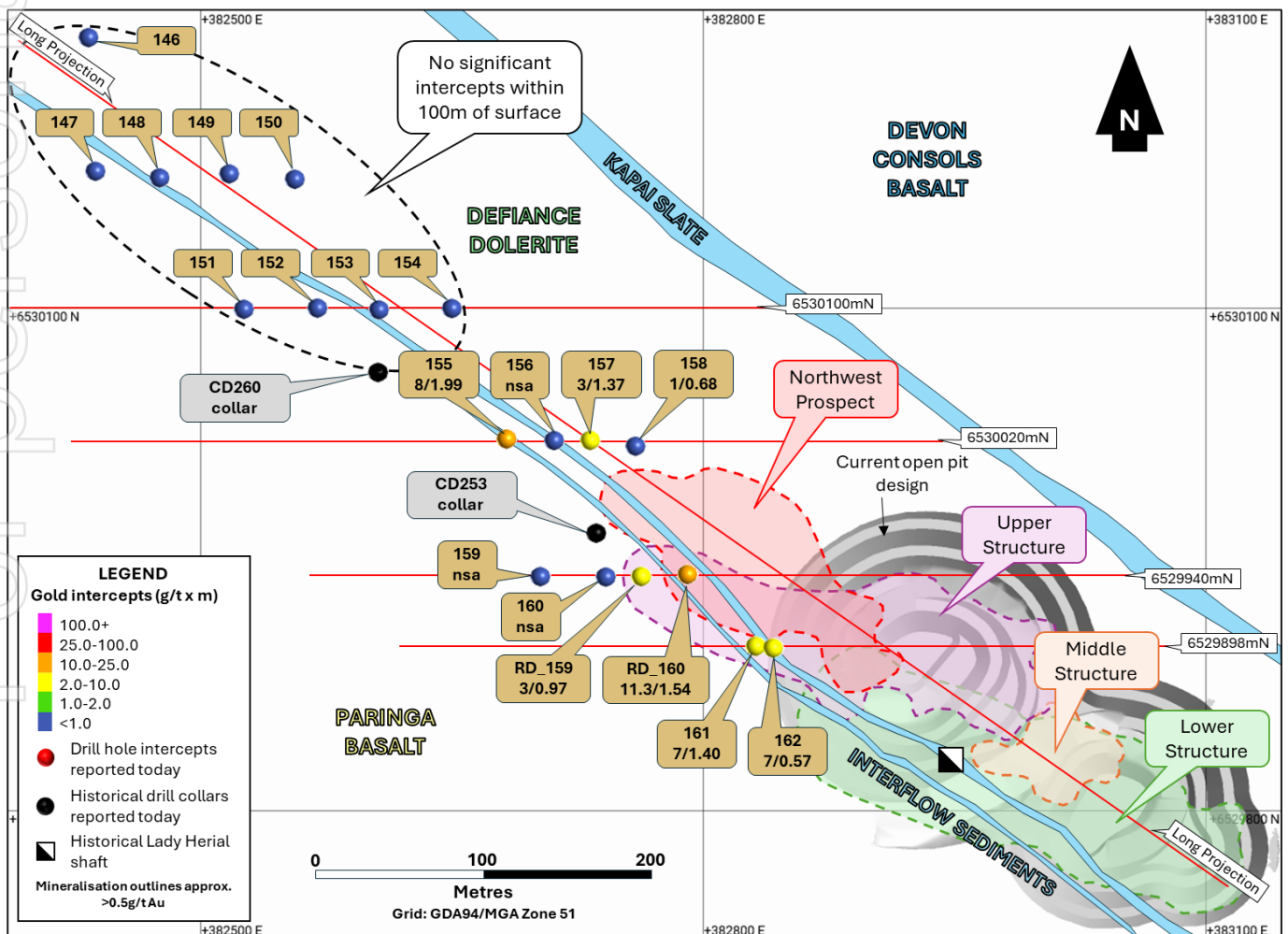
Figure 2: Plan view of the broader Lady Herial area showing today's results, the historical WMC holes (grey callouts) and location of the long section in Figure 3 and cross sections in Figures 4,5,6 and 7 .
