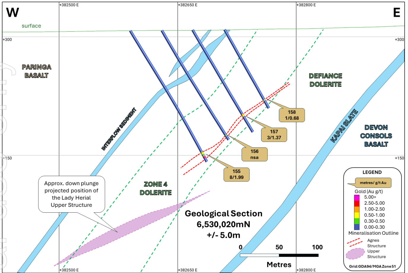
Figure 6: Cross section 6,530,020mN view of the Lady Herial area showing today's results.
