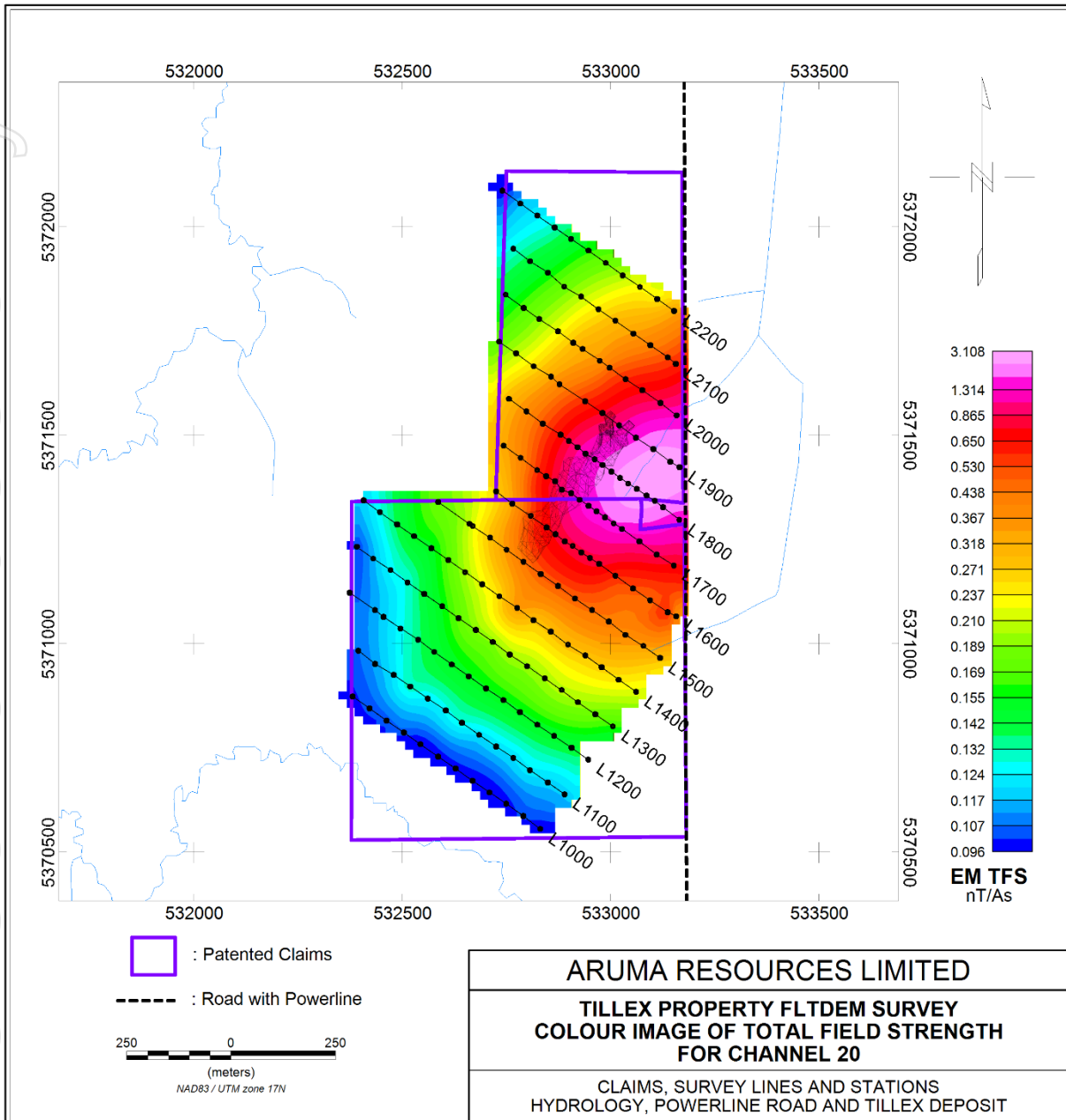
Figure 2: Plan view of EM Survey Modelled Contour Plan of the East Conductor with survey lines shown
