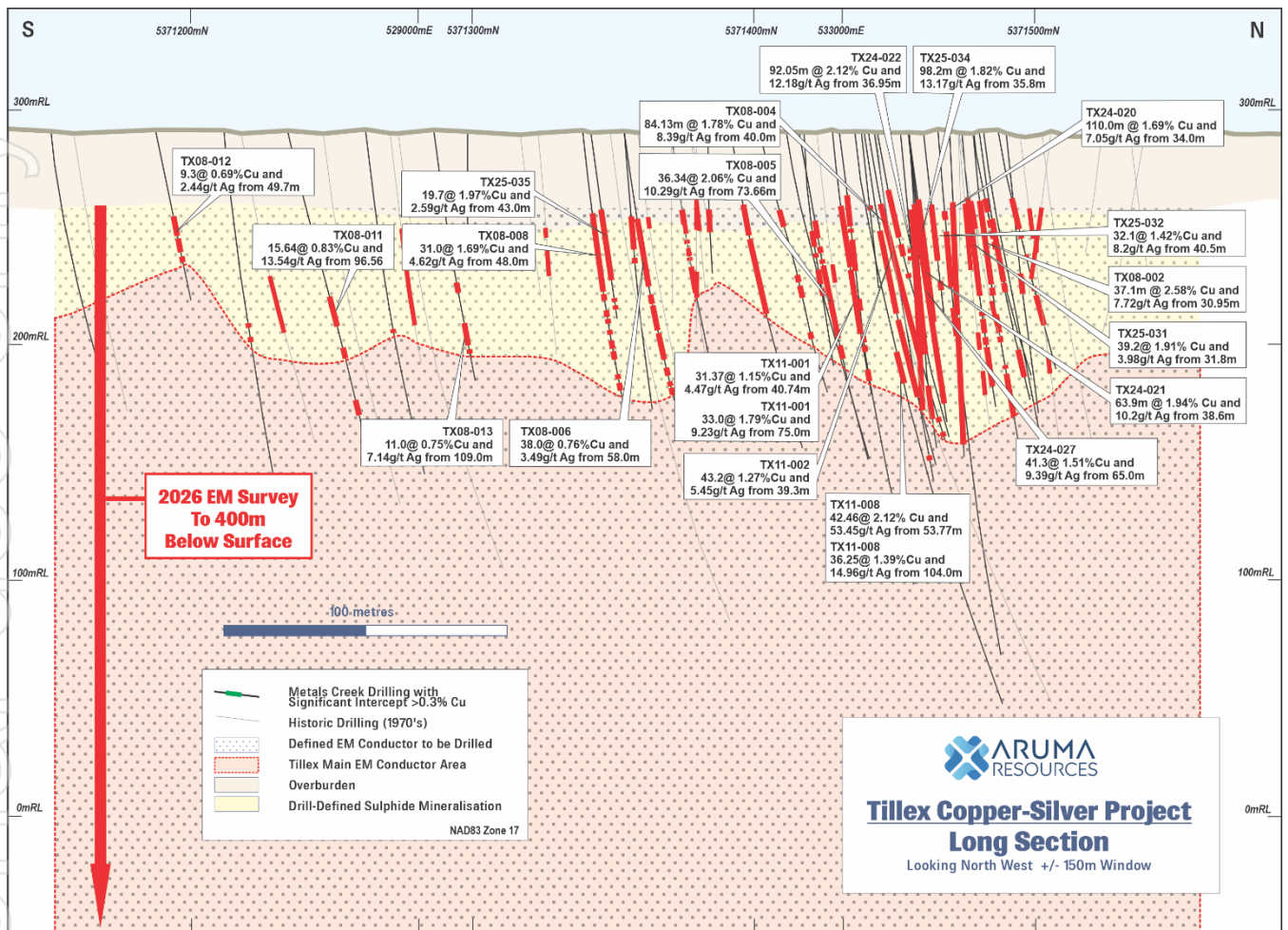
Figure 3: Long Section View of significant historic drilling intersections with the depth and strike extent modelled by the EM Survey at the Main Conductor (Refer Figure 1, Plan View)
