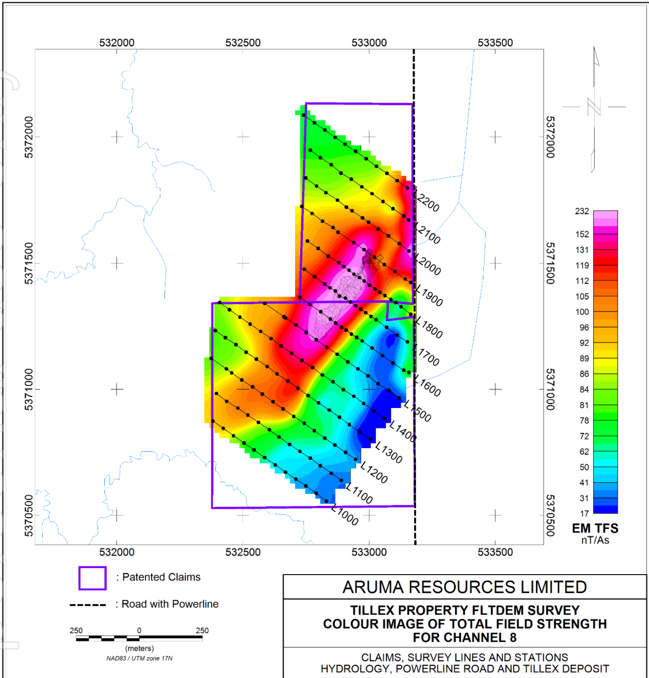
Figure 1: Plan view of EM Survey Modelled Contour Plan of the Main Conductor with survey lines shown
