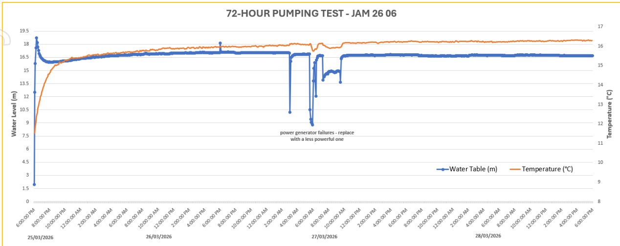
Figure 1. The graph shows the static water level dropping from 2m to 19m on startup to stabilising at 16.5m.
