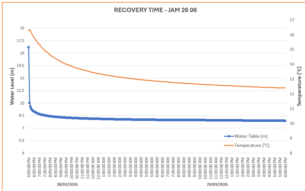
Figure 2. A sharp water level recovery was recorded immediately after shutdown (from 16.7m to ~10m).
