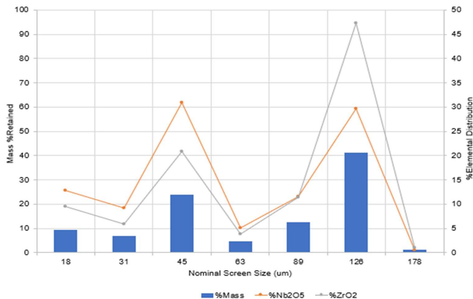
Graph 1-6: Bimodal Particle Size Distribution
