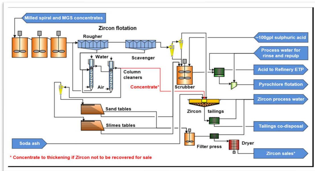
Figure 1-15: Proposed Zircon Flotation Flowsheet
