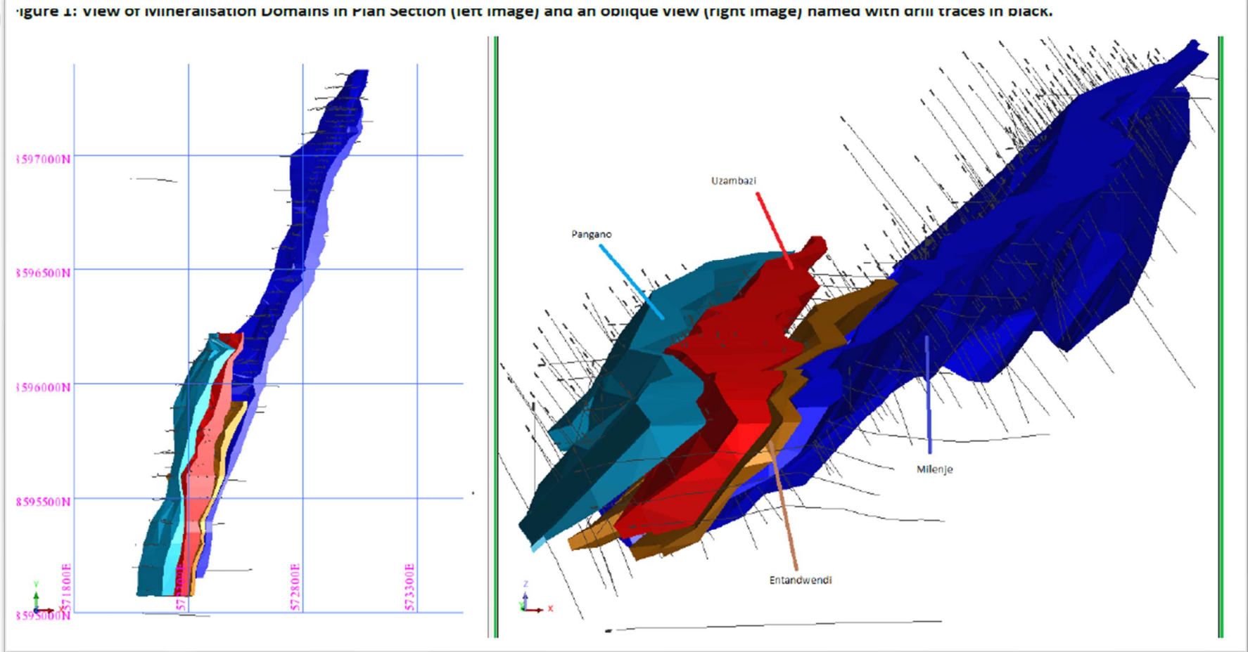
Figure 1-43: Mineralisation domains
