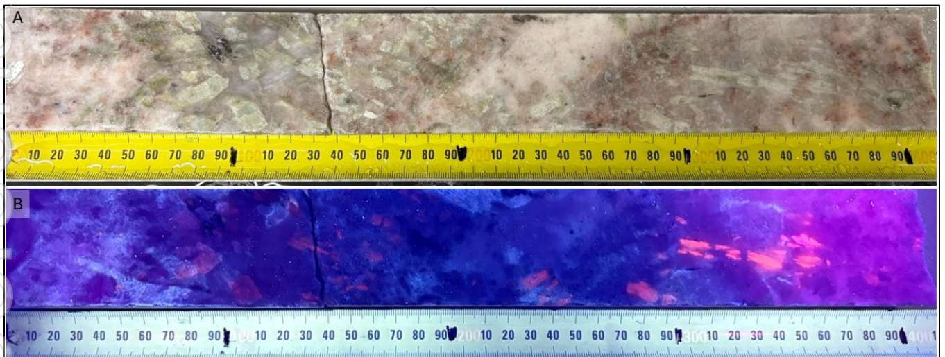
Figure 4: Top (A): Core from BCDD005 from 282.22m to 282.63m in natural light. Elongate white-green crystals are interpreted as spodumene. Bottom (B) The same core exposed to UV light confirming the elongate crystals fluoresce at a wavelength typical of spodumene (orange). Logged mineral abundance estimations provided (Table 4).
