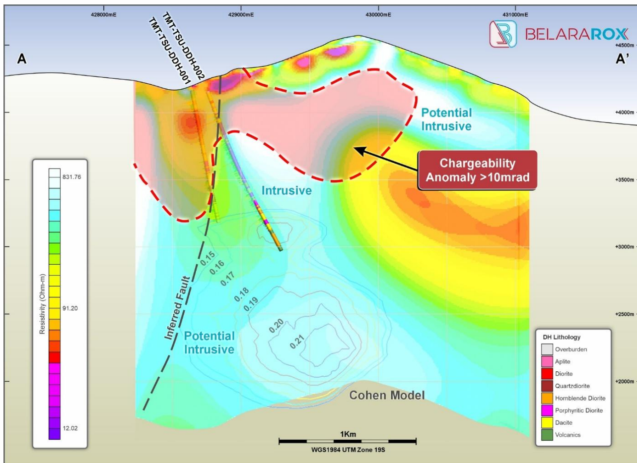
Figure 4. Cross-section A-A' (refer to Figure 3 for section location in plan view) of the Tambo South Target showing drill holes TMT-TSU-DDH-001 and TMT-TSU-DDH-002 from the 2025 field season drilling 5 , chargeability and resistivity anomalies from the recently completed MT/IP survey and geochemical anomaly. Note: The numbers on the iso surfaces represent probability scores (0.0-1.00) of the geochemical models at Toro South matching with the reference metal-zoning models from Cohen (2011). Values over 0.15 are considered 'significant', with a maximum score of 1.00, which corresponds to a 100% match.
