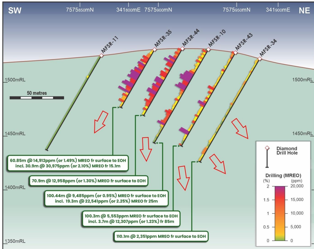
Figure 1 Cross-section showing significant weighted average MREO. Section looking northwest, H/V is 1:1 and location in Figure 2.
