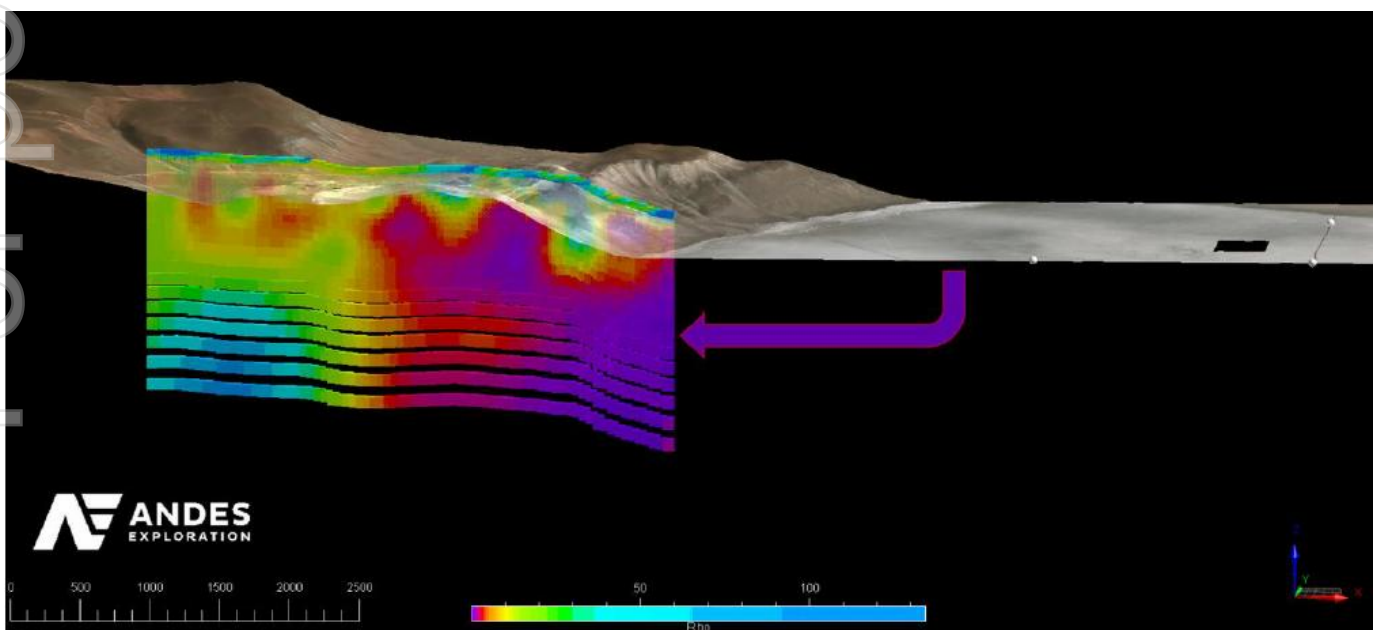
Figure 2 – Cross Section (L1000) Highlighting Depth-Continuous Conductive Zone Interpreted as a Brine Target
