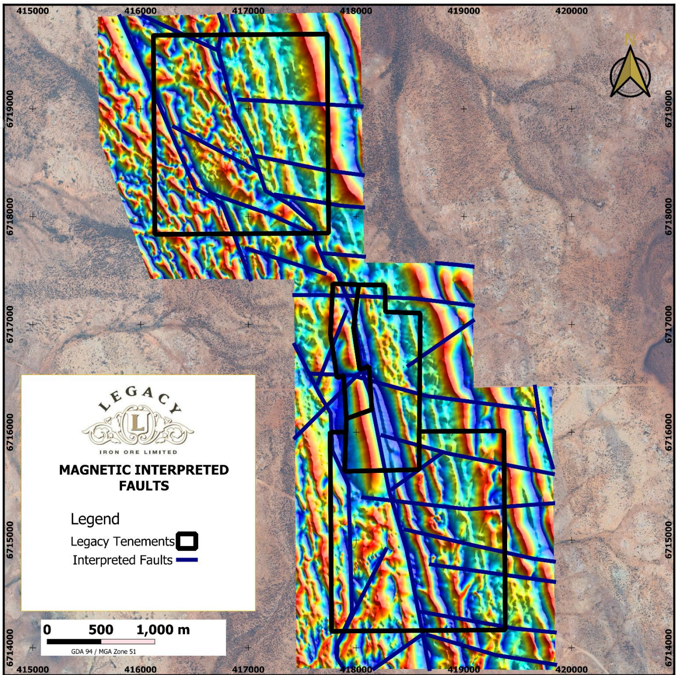
Figure 3. Yilgangi structural interpretation overlaid onto the RTP Tilt Derivative image.
