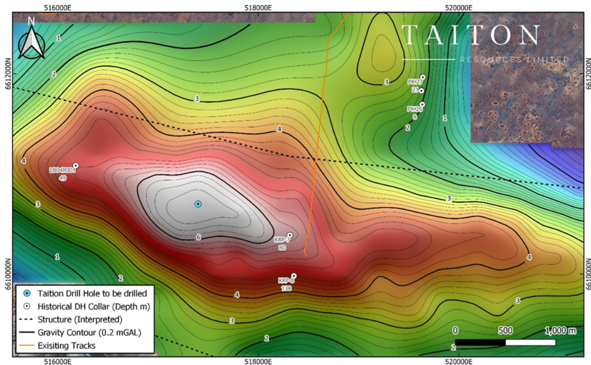
Figure 2. Drill hole collar location with gravity contours underlain by residual Bouguer gravity anomaly image.
