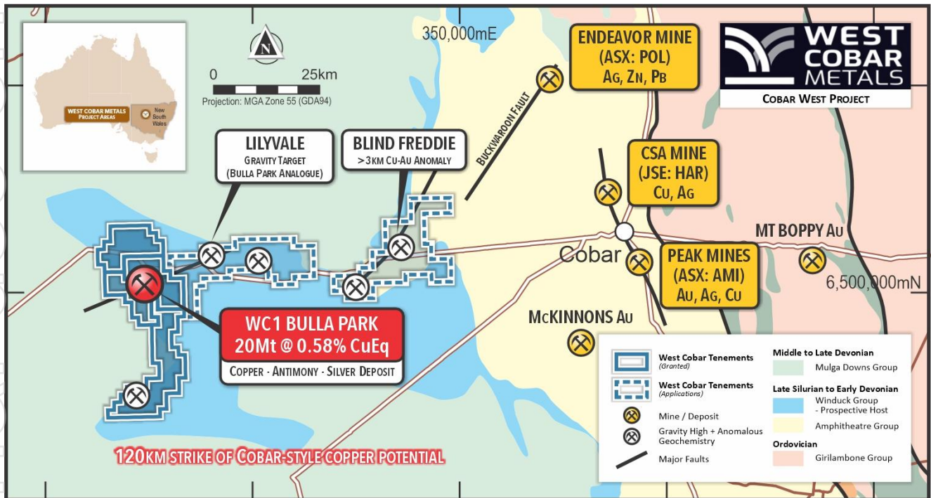
Figure 2: Cobar Basin showing West Cobar Metals' district-scale position, tenements and recent ground applications, Bulla Park deposit and other significant deposits of the Cobar Basin
