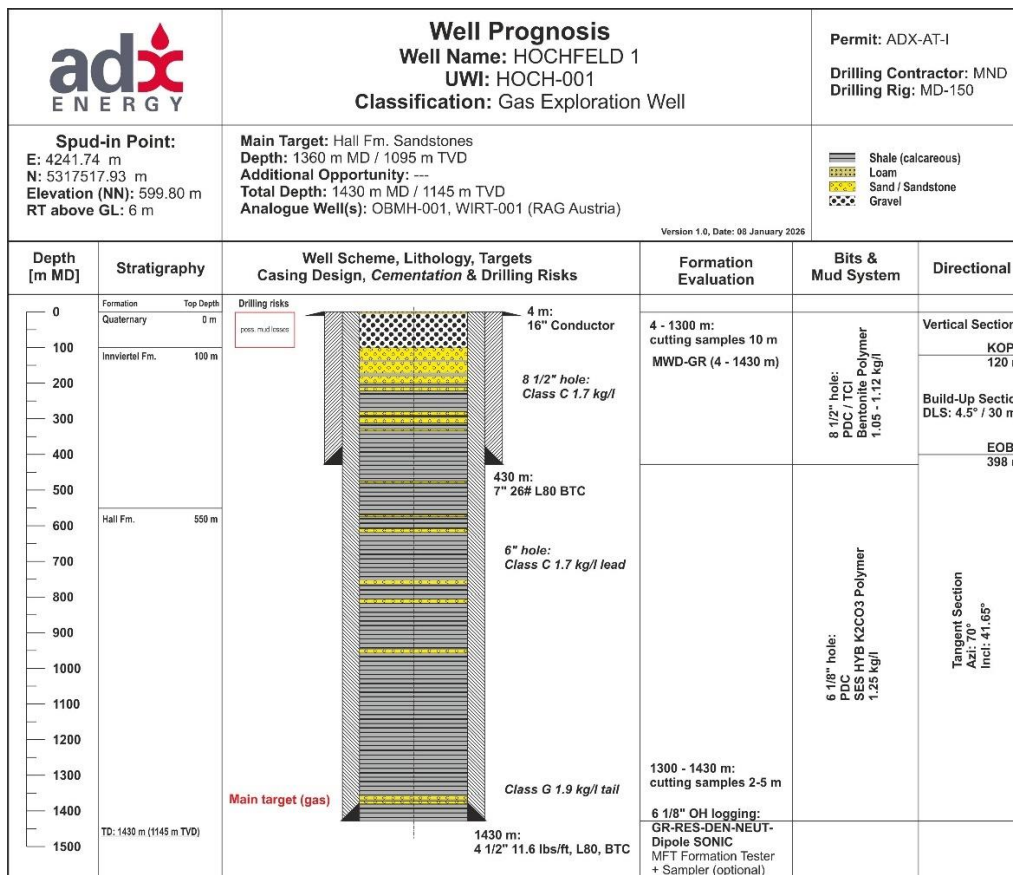
Figure 5: HOCH-1 Well Plan
