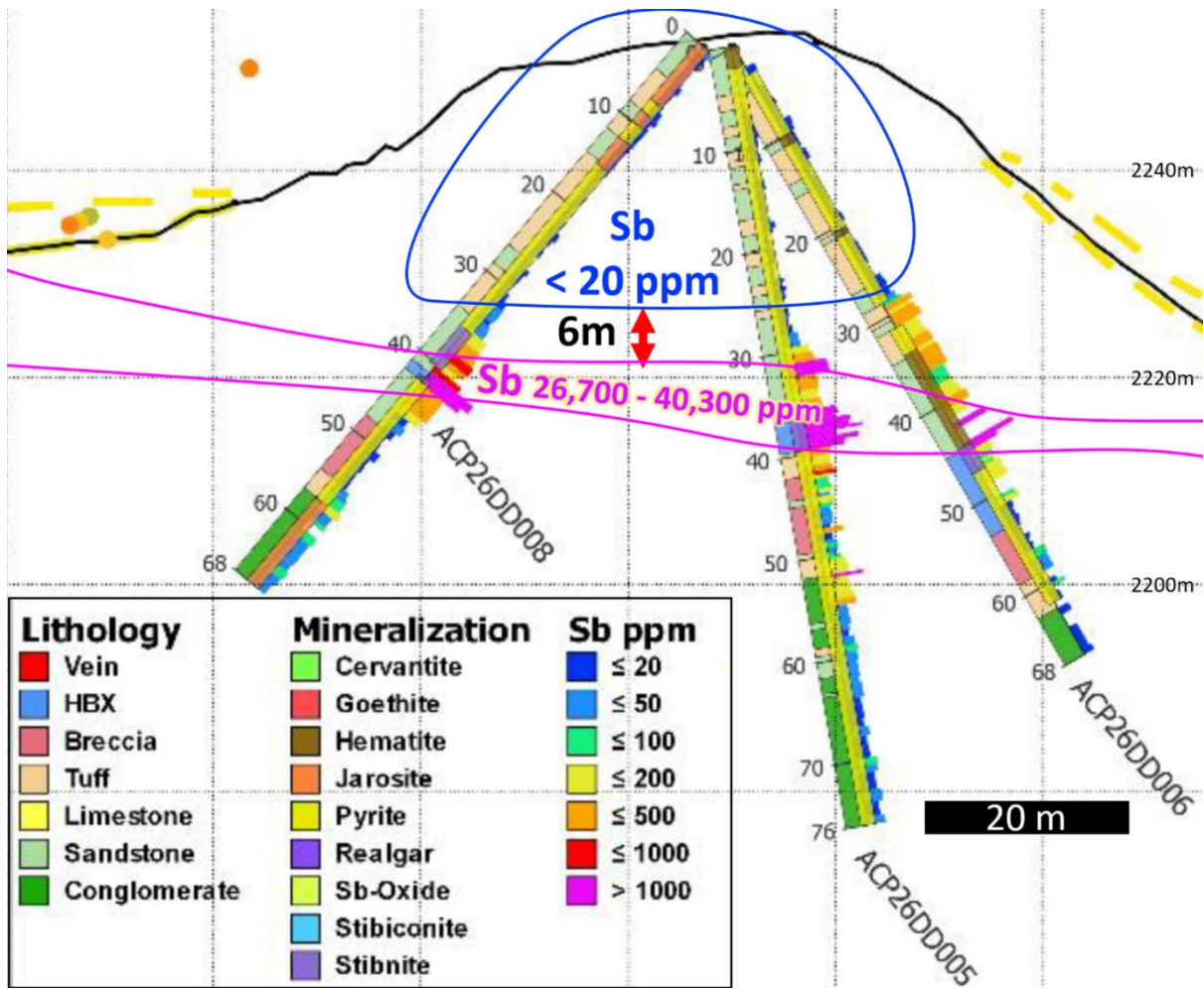
Figure 2*: Antimony mineralisation in AT4 Drill holes 5,6 and 8. Sb halo below 20 ppm occurs 6m above the highly mineralised zone. Thus, Sb concentrations between 2-26 ppm (at Dry Wash) may be indicative of proximity to ore-grade Sb deposits. Pyrite (marcasite), hematite and goethite are also observed in GGE's leases, also shown here above and proximal to Antimony Canyon Sb ore zones. *Original figure modified from Figure 4 in AT4:ASX March 10, 2026 announcement [1].
