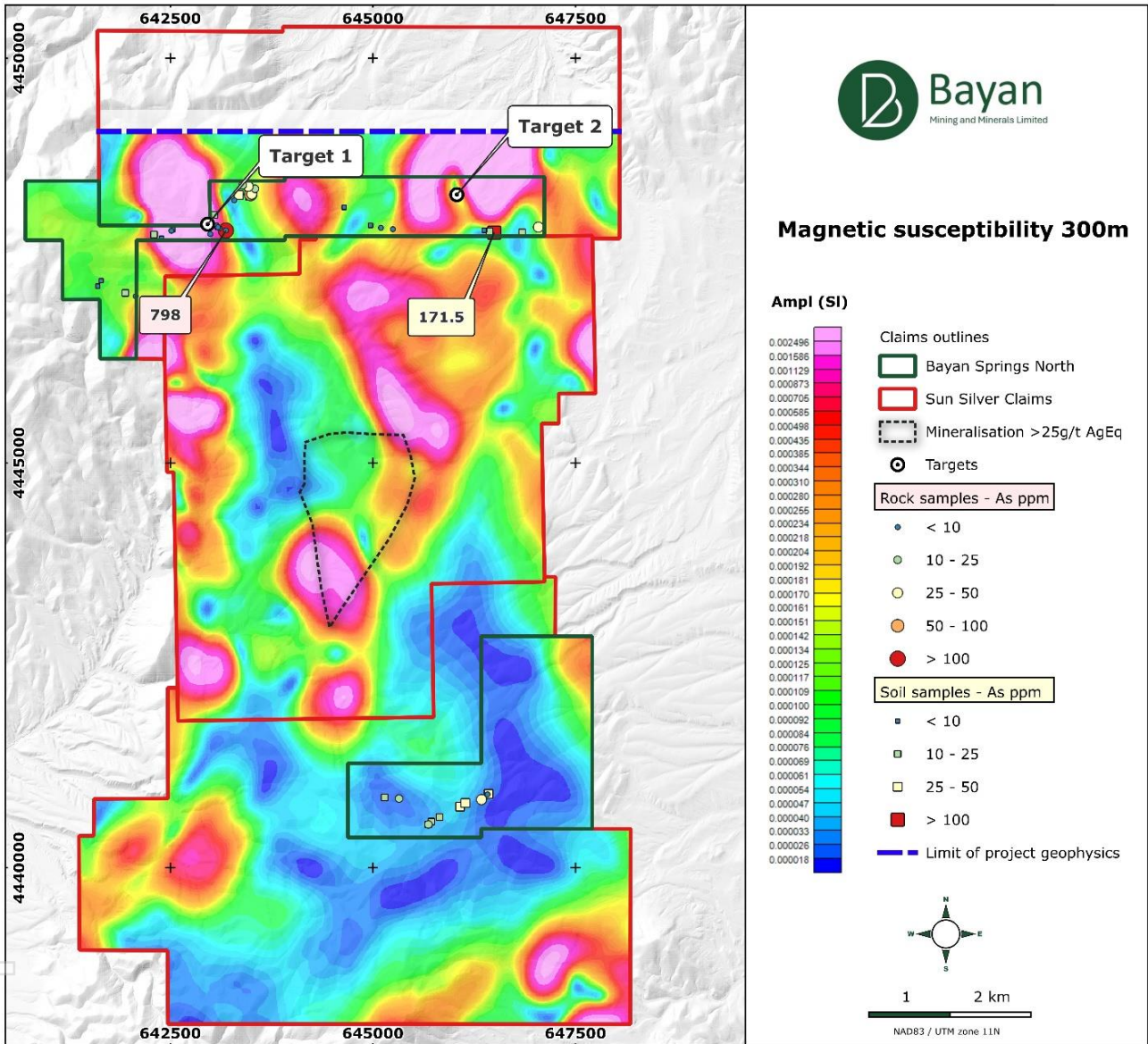
Figure 2: Modelled Magnetic Susceptibility at 300m Depth
