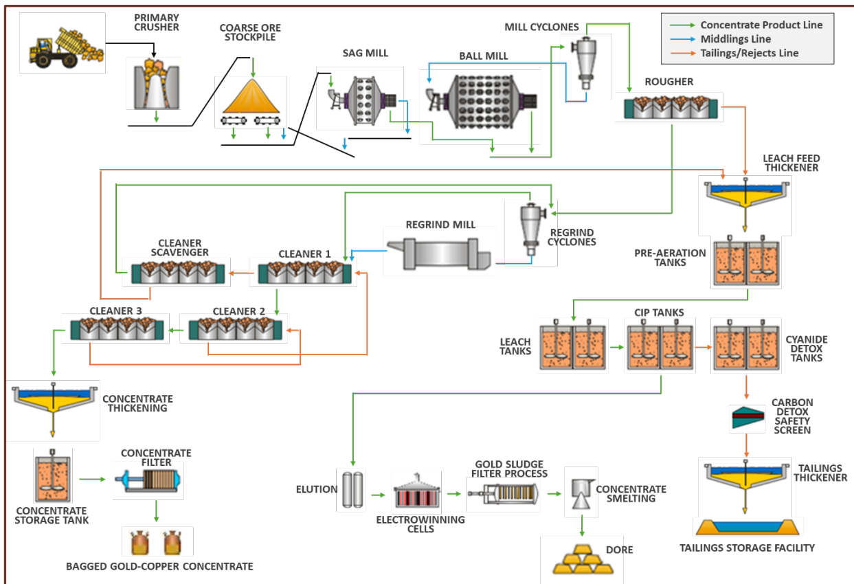
Figure 6. Bramaderos process route flowsheet.
