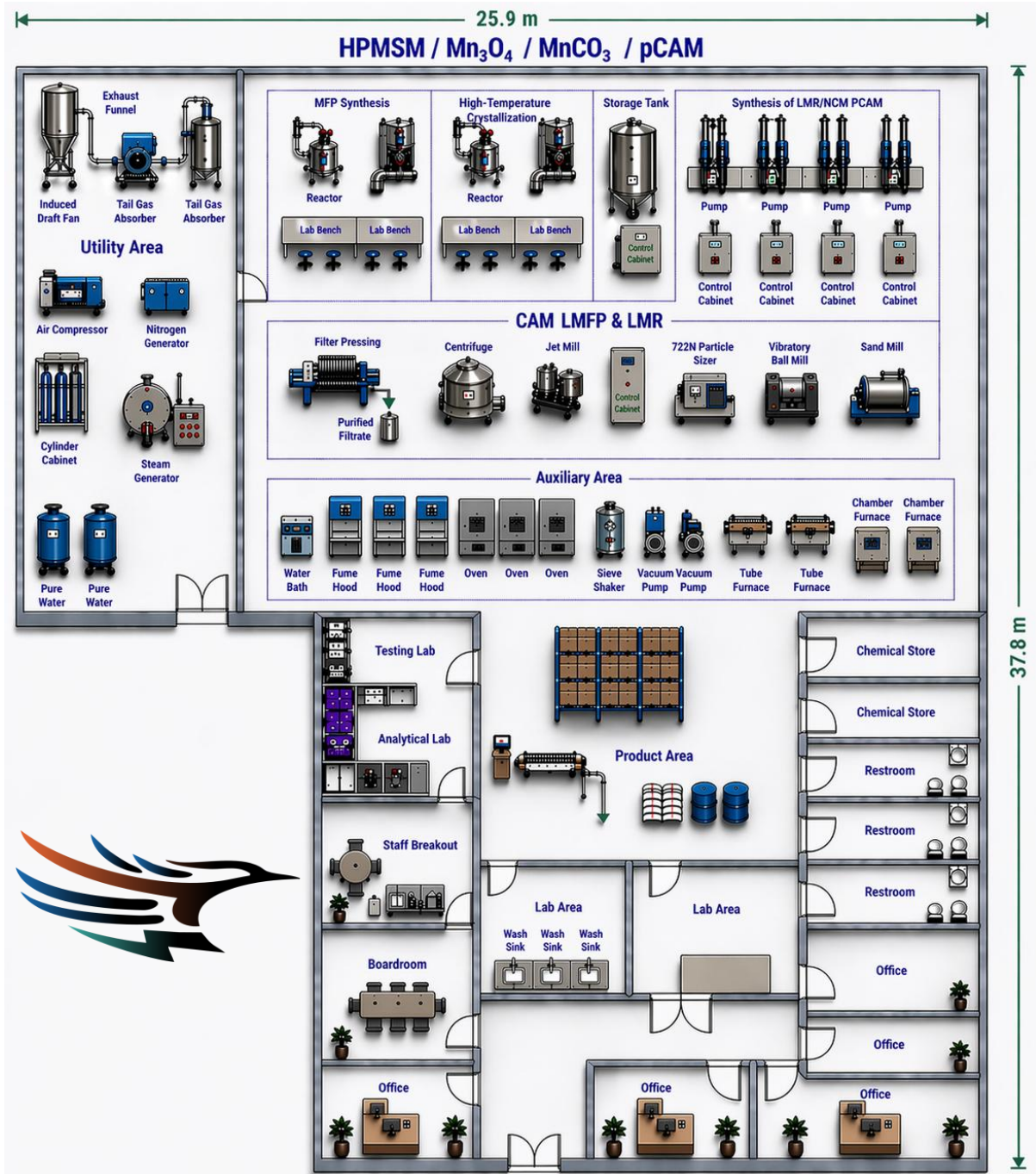
Figure 1. Model diagram and layout of the proposed Australian Demonstration Plant (ADP) to be constructed in Perth, Western Australia.
