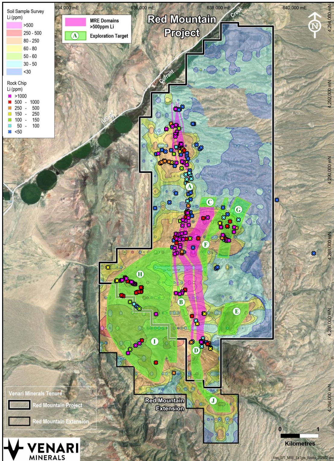
Figure 9. Rock chip geochemistry, MRE and Exploration Target Areas over gridded soil sample geochemistry image
