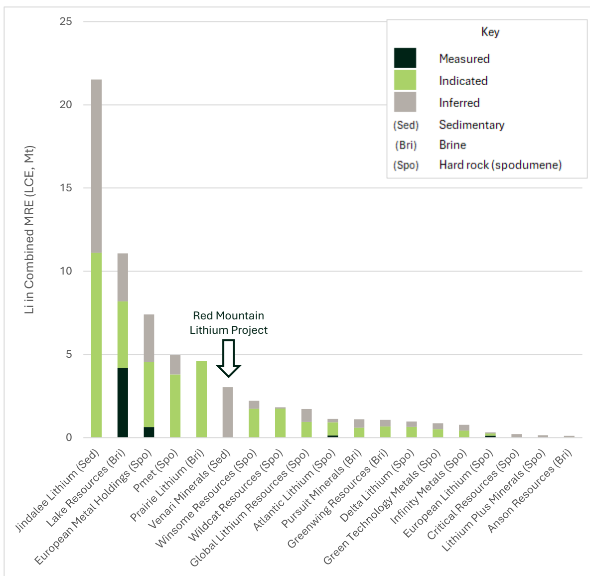
Figure 6. ASX-listed lithium explorer (producers and developers excluded) ranked by contained Lithium Carbonate Equivalent (LCE) by Mineral Resource Category and deposit type. Contained LCE calculated using 2.475 conversion factor for Li 2 O – LCE and 5.323 conversion factor for ppm Li to LCE. Source MRE details provided in Table 6
