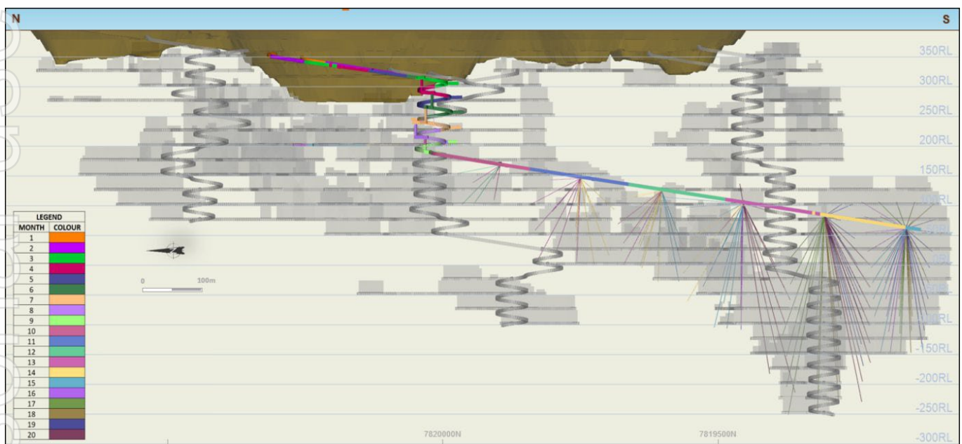
Figure 2: Planned Exploration Decline at Groundrush. View looking east.
