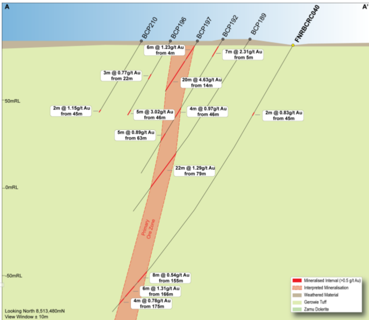
FIGURE 1: CROSS SECTION (A-A'): PRIMARY ORE ZONE - LOOKING NORTH ±10M SECTION VIEW, SHOWING INTERPRETED GEOLOGY AND SIGNIFICANT INTERSECTIONS (AU >0.50G/T). DRILLING RESULTS ARE DOWNHOLE WIDTH AND NOT TRUE WIDTH
