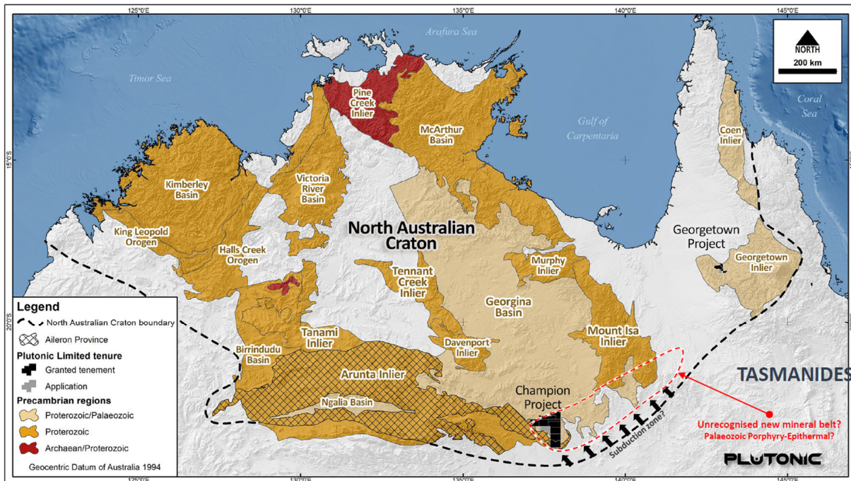
Location of the Plutonic Champion Project, located within the Northern Territory along the Queensland border. Plutonic targeted the area on their interpretation of a favourable tectonic setting (shown) that has not been tested for gold-copper mineral systems previously.
